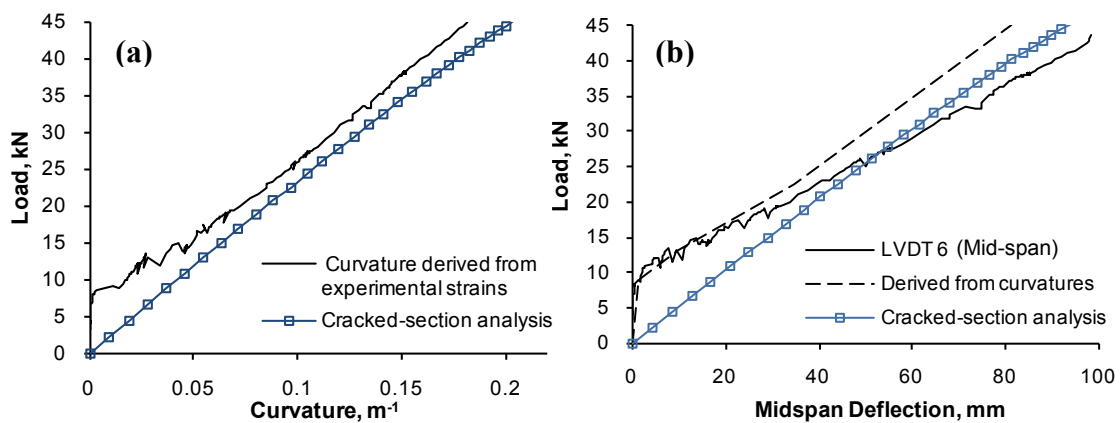
Figure 5. Typical experimental load vs. (a): curvature, and (b): mid-span deflection, slab SG2a
