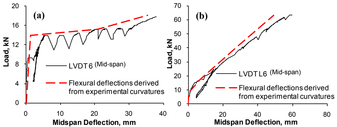
Figure 8. Experimental load vs. mid-span deflection for (a): SG1, and (b): SG3
