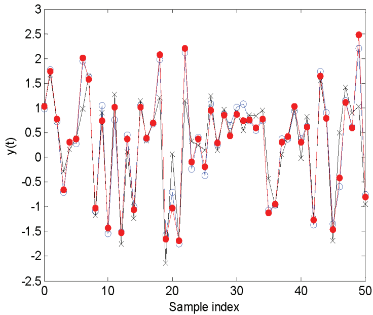
Figure 5. A comparison of the model predicted outputs produced by the identified polynomial and wavelet models, with the true values produced by the noise-free model (22), driven by the input in the first test case described in Example 1. Circles present the true values, dots present the model predicted output from the wavelet model, and crosses present the model predicted output from the polynomial model.
