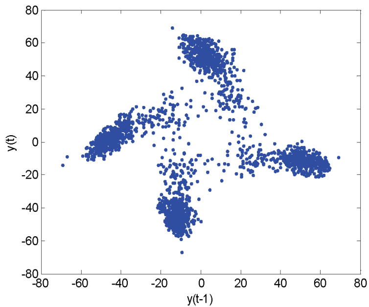
Figure 12. The first return map produced by the model predicted output of 2000 data points from the identified polynomial model, driven by a random sequence that was uniformly distributed in [-5,5] .
