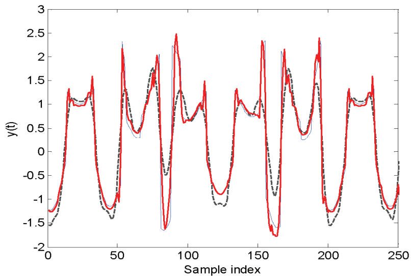
Figure 6. A comparison of the model predicted outputs produced by the identified polynomial and wavelet models, with the true values produced by the noise-free model (22), driven by the input in the second test case described in Example 1. The thin solid line presents the true values, the thick solid line resents the model predicted output from the wavelet model, and thick dashed line represents the model predicted output from the polynomial model.
