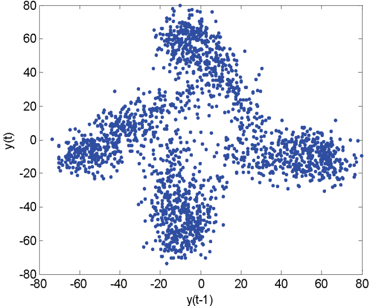
Figure 9. The first return map formed by the 2000 noisy training data points generated by model (28) in Example 3.
