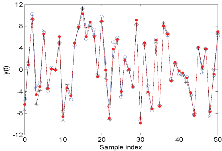
Figure 8. A comparison of the model predicted outputs produced by the identified polynomial and wavelet models, with the true values produced by model (25), described in Example 2. Circles present the true values, dots present the model predicted output from the wavelet model, and stars present the model predicted output from the polynomial model.
