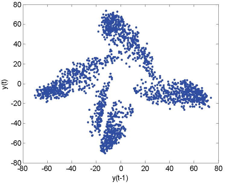
Figure 10. The first return map form by the associated noisy-free data (2000 points) generated by model (28) in Example 3.
