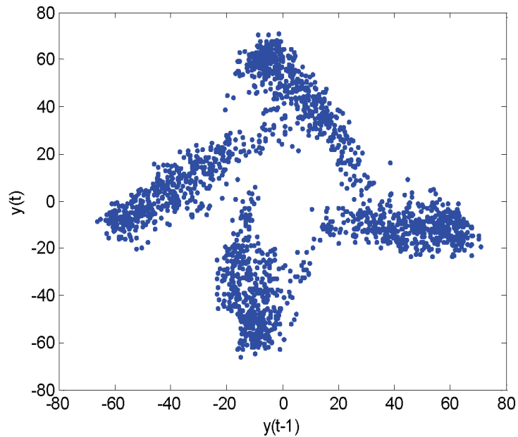
Figure 13. The first return map produced by the model predicted output of 2000 data points from the identified wavelet model, driven by a random sequence that was uniformly distributed in [-5,5] .
