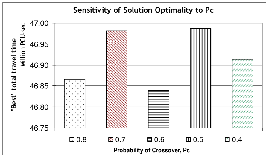
(a) Optimality of final solution
