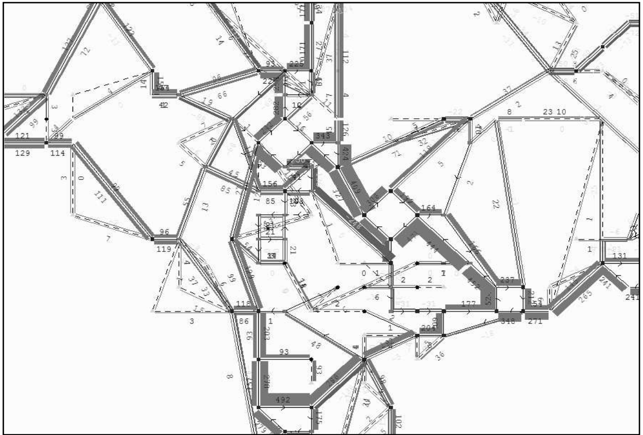
FIGURE 10: Difference in link flows as a result of SATOPT timings (pcu/hour)
