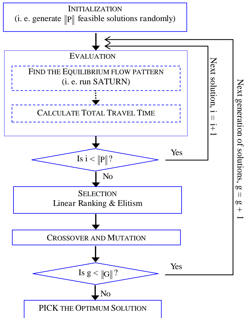
FIGURE 2 GA-FITSUM Flow Chart
