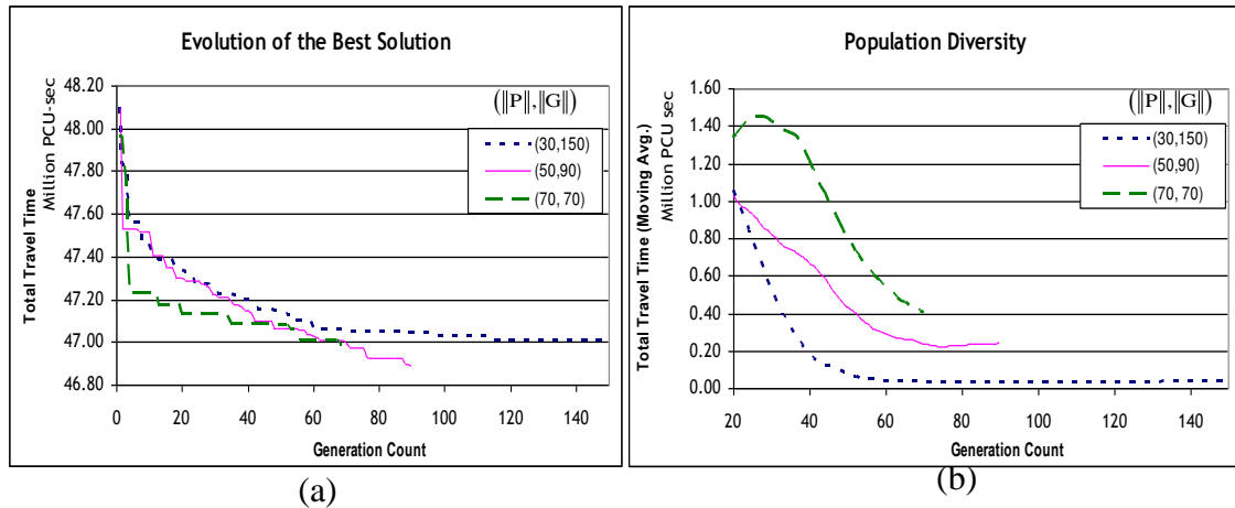
FIGURE 6: Comparison of different (\|P\|, \|G\|) values
