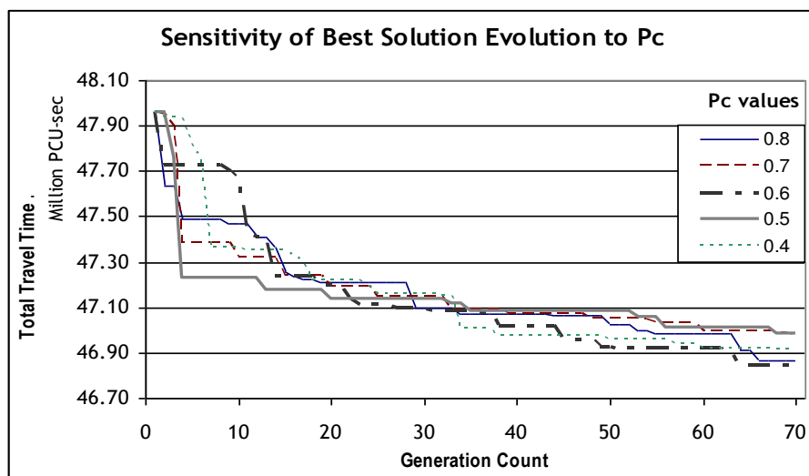
(b) Profile of improvement of best solution
