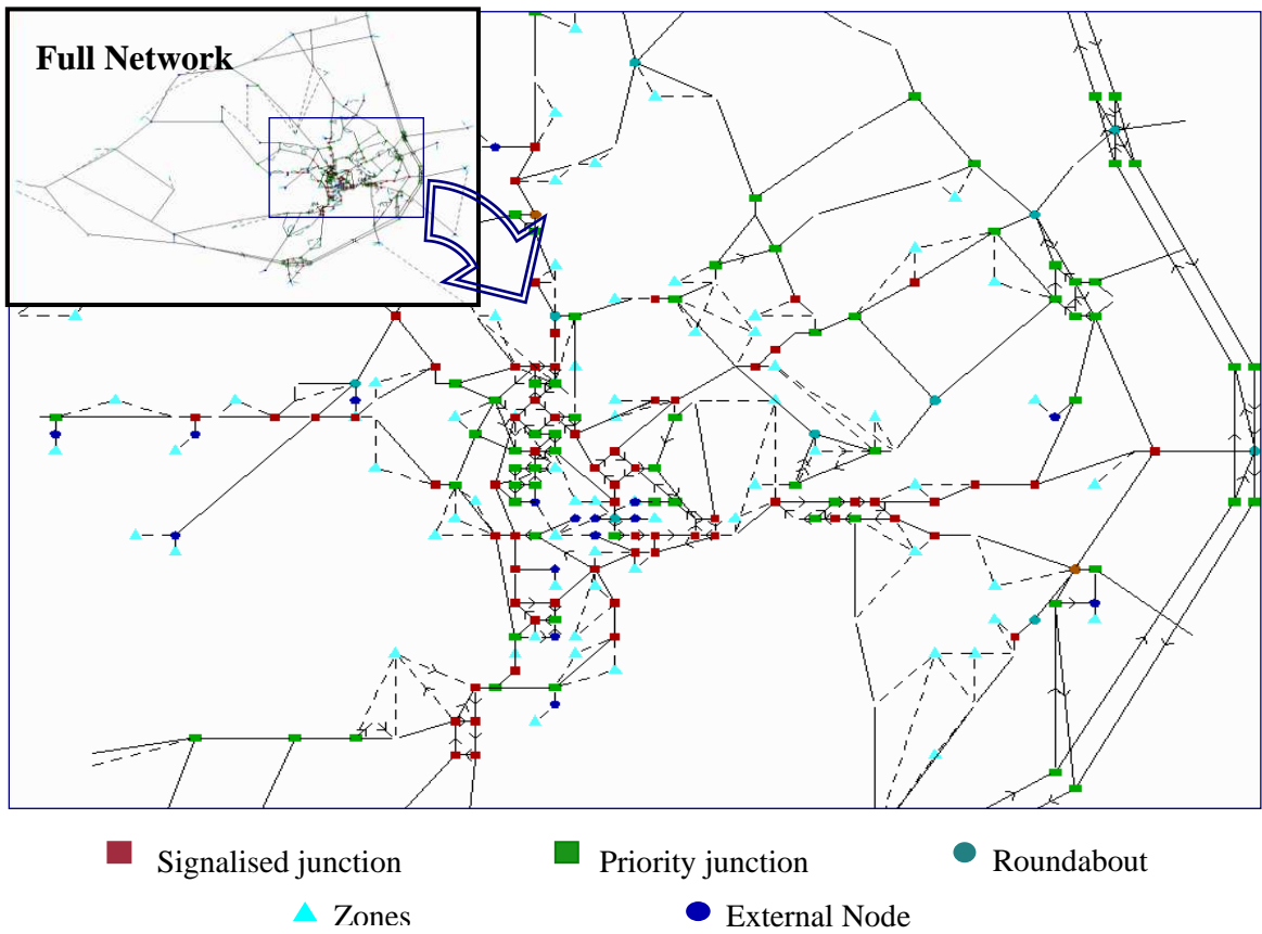
FIGURE 5: Layout of the Chester network
