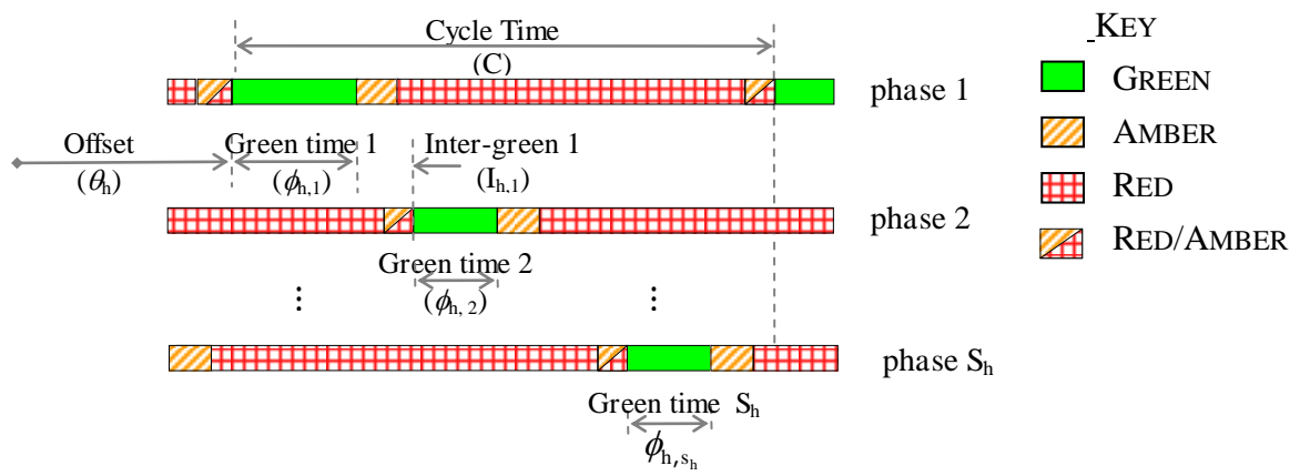
FIGURE 1 Signal design variables for junction h
