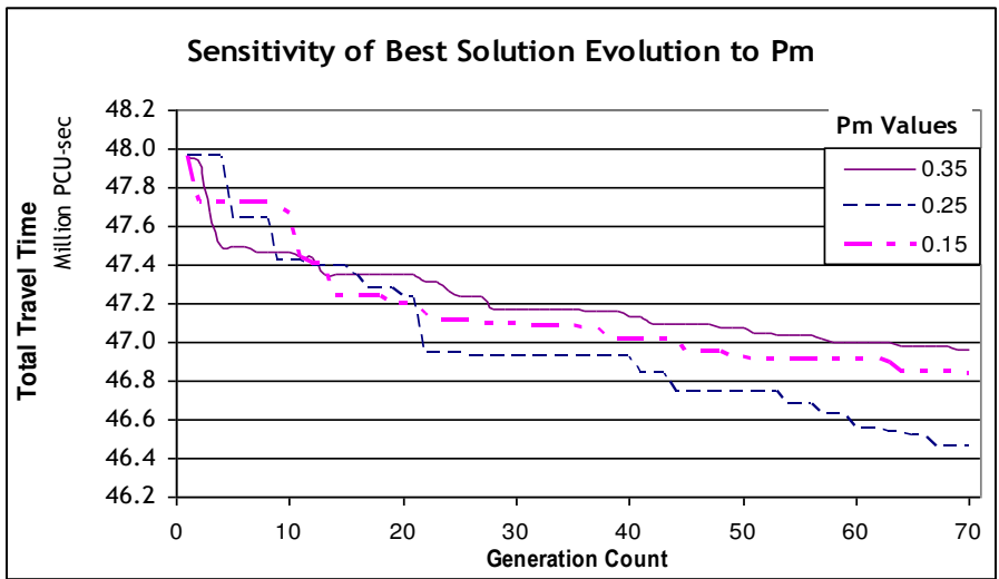
(b) Profile of improvement of best solution
