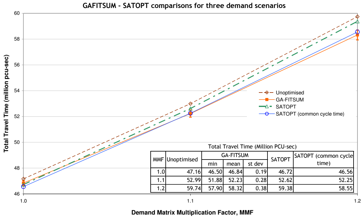
Figure 9 Total travel time comparison of SATOPT and GA-FITSUM
