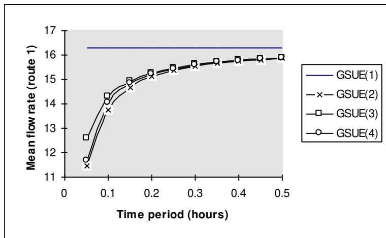
Figure 1: GSUE( n ) mean flow rate on route 1 ( n=1,2,3,4 ) as a function of time period duration \tau
