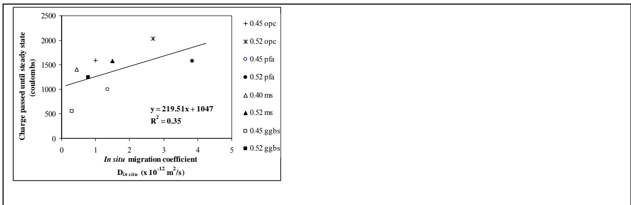
Fig. 10 - Relationship between D_{in situ} and the charge passed until steady state in Permit ion migration test. The graph only reports data from 28 day and 56 day tests.
