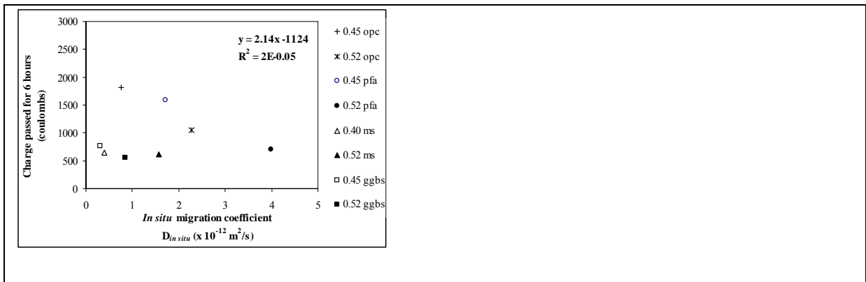
Fig. 9 - Relationship between D_{in situ} and the charge passed during the initial 6 hours in Permit ion migration test. The graph only reports data from 28 day and 56 day tests.
