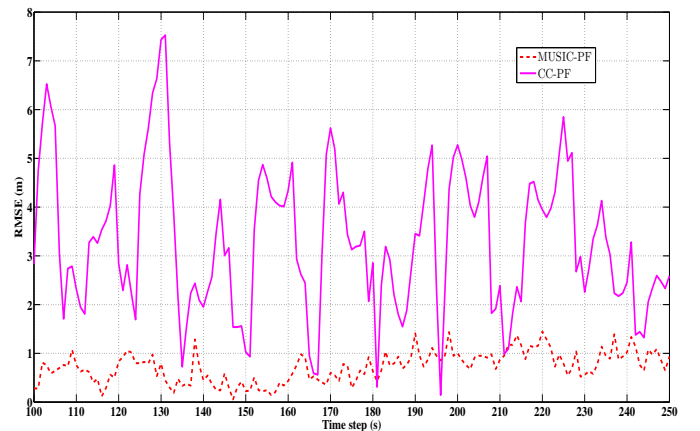
Figure 2. RMSE comparison between MUSIC-PF and CC-PF algorithm.
