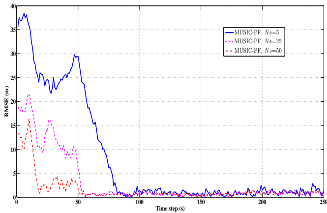
Figure 3. RMSE comparison of MUSIC-PF for different number samples.
