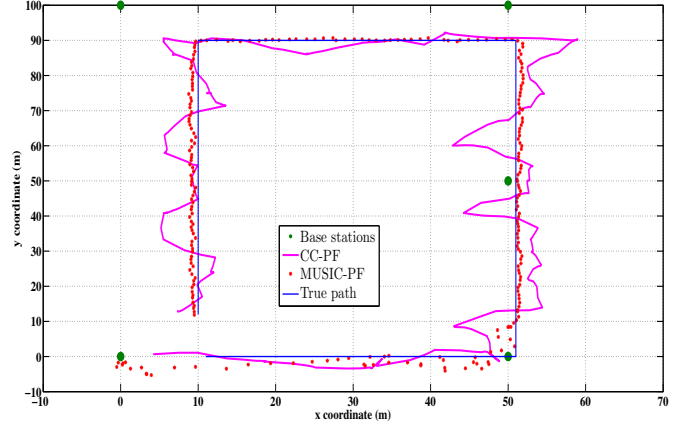
Figure 1. Comparison between MUSIC-PF and CC-PF techniques.
