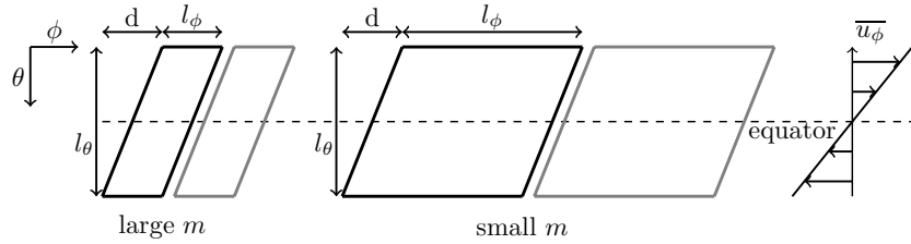
Figure 13: Schematic representation of latitudinal velocity contours (black: positive and gray: negative) in a plane (\phi, \theta) for two modes of different azimuthal order m .
