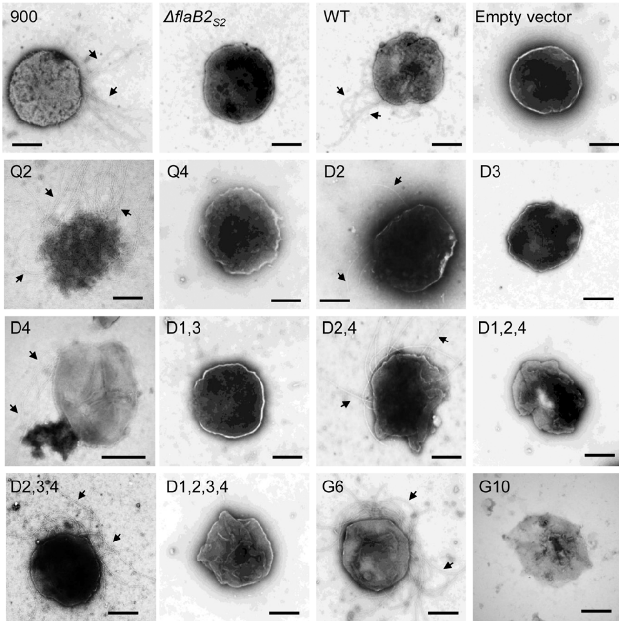
Fig 3. Transmission electron micrographs of select \Delta flaB2_{S2} strain complemented with flaB2_{S2} with mutations at various N-glycosylation sites. Wildtype Mm900 cell (900) was archaeellated, while the \Delta flaB2_{S2} mutant was not. Wildtype FlaB 2S2 protein expressed in \Delta flaB2_{S2} restored archaeellation (WT), but the empty vector could not. Archaella were observed on surface of Q2, D2, D4, D2,4, D2,3,4 and G6 complemented cells. Cells complemented with Q4, D3, D1,3, D1,2,4, D1,2,3,4 and G10 were non-archaeellated. Archaella are indicated by arrows. Bar equals 500 nm.
