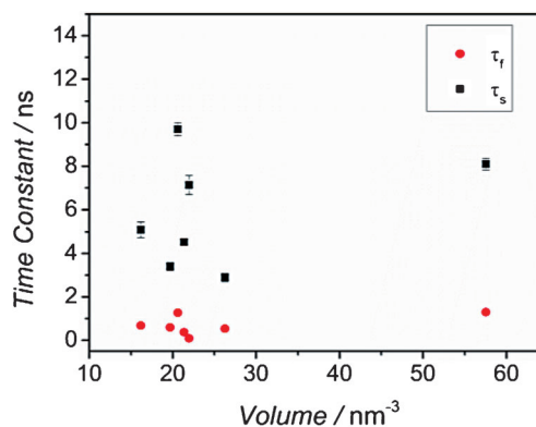
Figure 5. Fast and slow time constants for different unpassivated samples in respect to the volume.
