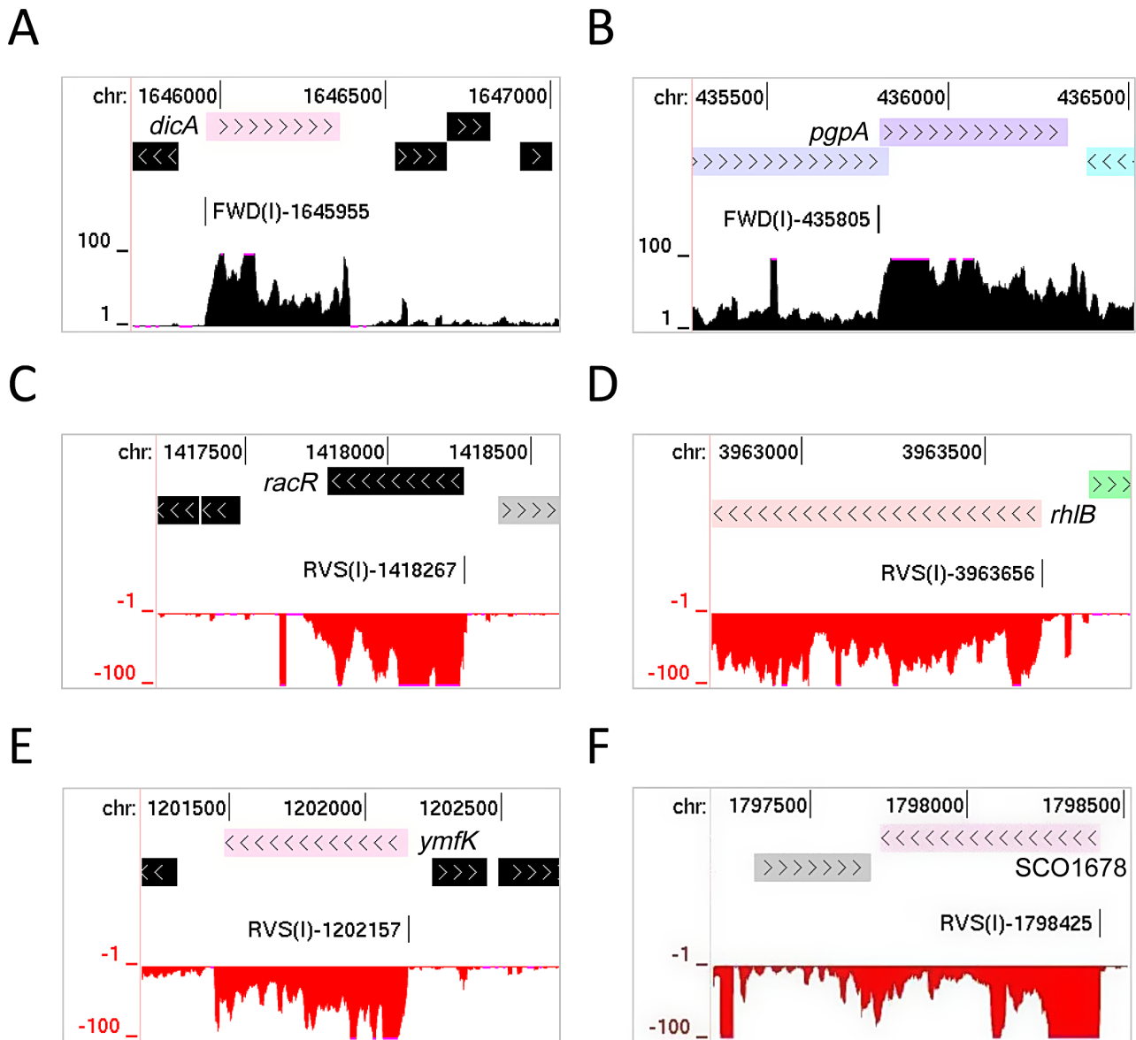
Fig. 2. Examples of leaderless mRNAs. (A), (B), (C), (D) and (E) correspond to E. coli genes dicA (Qin prophage; b1570), pgpA (b0418), racR (Rac prophage; b1356), rhlB (b3780) and ymfK (e14 prophage; b1145) respectively. (F) corresponds to an unnamed paralogue (SCO1678) of the S. coelicolor gene whiH . The panels are modified screenshots from the UCSC Microbial Genome Browser (Chan et al. , 2012). In each panel the tracks depict from top to bottom, the genome position, location of annotated genes, the positions of TSSs identified by the analysis of M-A scatterplots (Fig. 1), and the number of times each position on the corresponding strand was sequenced following fragmentation of the transcriptome (gRNA-seq). The numbers at the left of the RNA-seq tracks indicate the scale of the sequencing reads.
