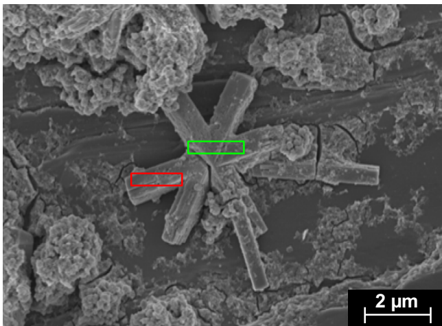
Fig. 11. Scanning electron microscope image used during electron dispersive spectroscopy analysis. The image illustrates zirconium citratomolybdate at 336 h into the synthesis. The EDX main parameters: working distance at 8 mm; electron intensity at 20 keV.
