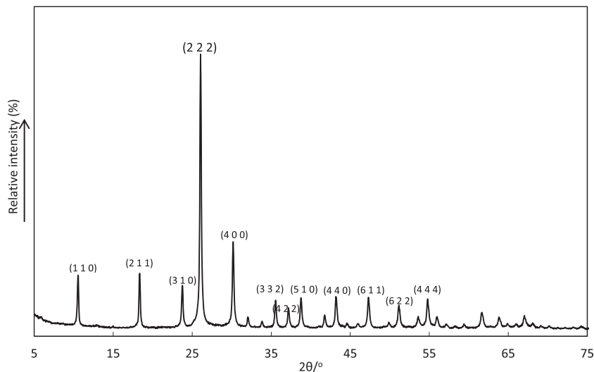
Fig. 15. X-ray diffraction pattern for caesium phosphomolybdate.
