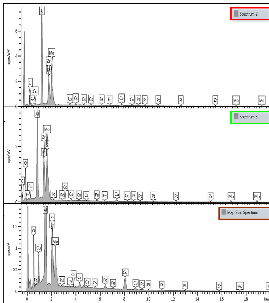
Fig. 12. Electron dispersive spectroscopy point and identification method. The image illustrates the spectrum of specific locations of the sample (spectrum 2 and 3) and a mass spectrum of both locations.
