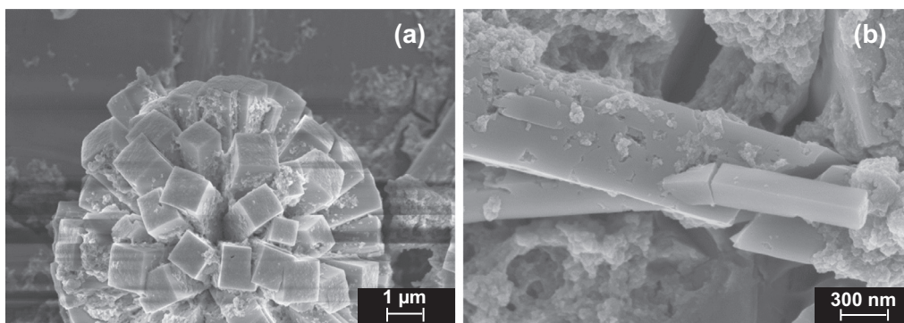
Fig. 9. Scanning electron images illustrating the formation of zirconium citratomolybdate, 192 h into the synthesis. The images were taken at different magnifications: (a) contact twinning at 29.63 K; (b) penetration twinning at 125.70 K.
