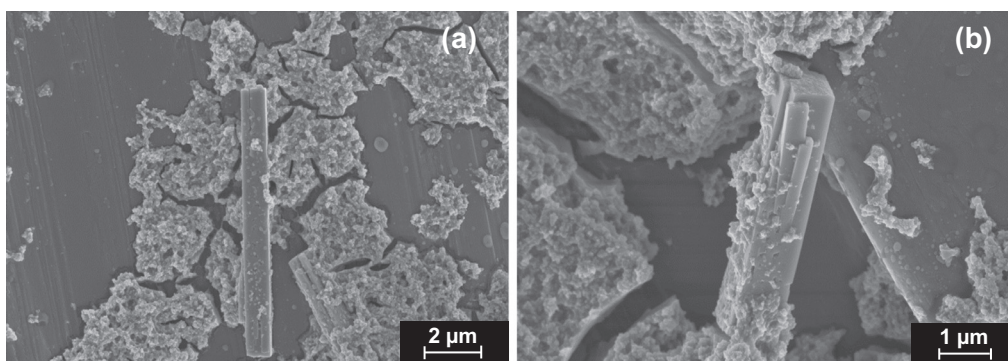
Fig. 10. Scanning electron images illustrating the formation of zirconium citratomolybdate, 336 h into the synthesis. The images were taken at different magnifications: (a) fully developed zirconium citratomolybdate at 21.02 K; (b) step growth of crystals at 37.63 K.
