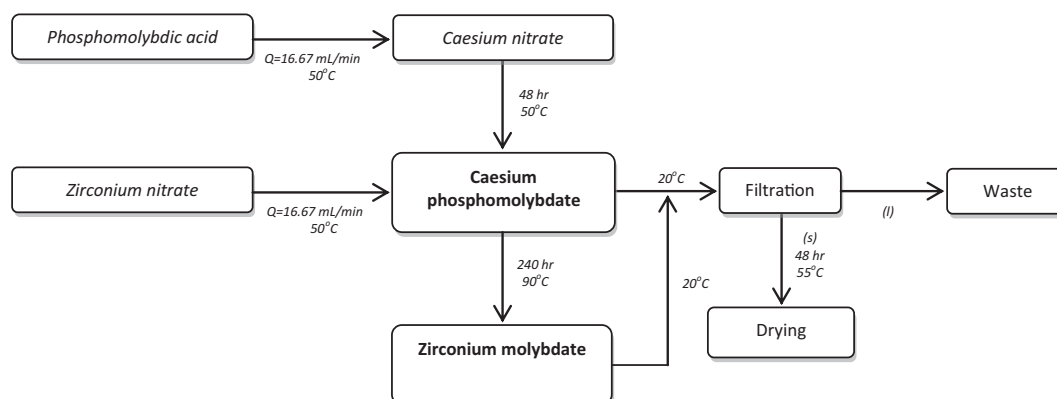
Fig. 2. Schematic illustration of the synthesis steps for caesium phosphomolybdate and zirconium molybdate particle production.
