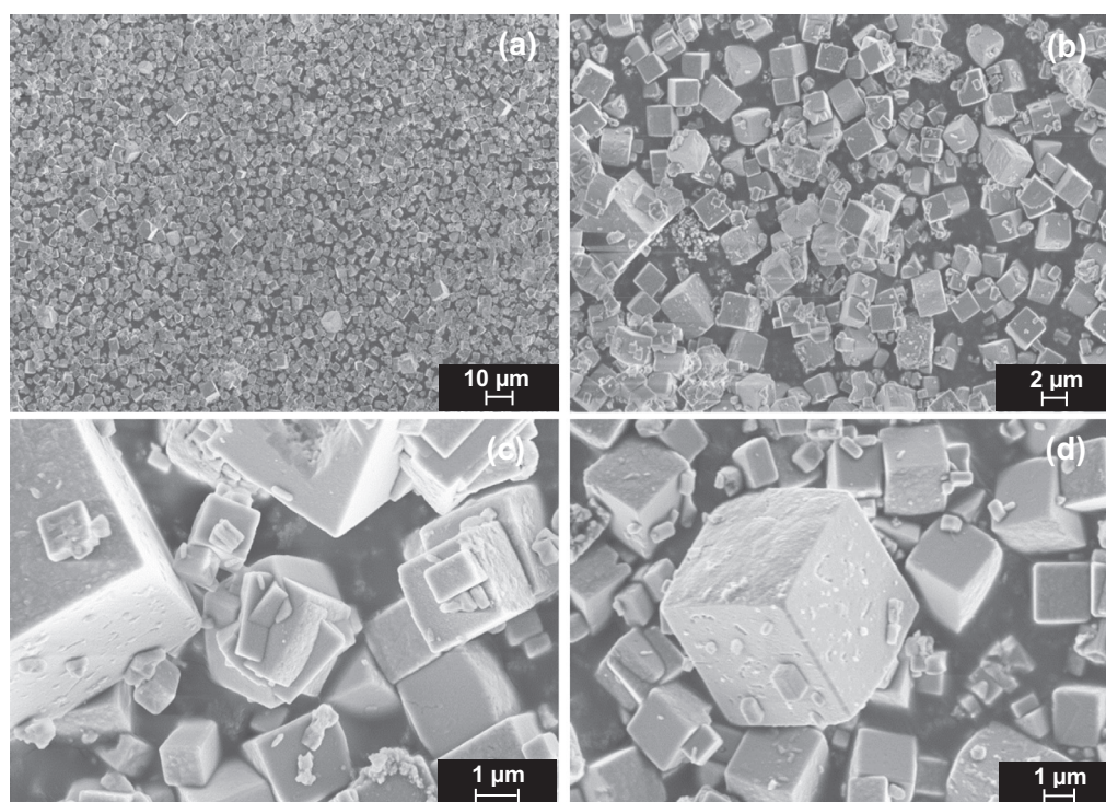
Fig. 7. Scanning electron microscope images of synthesised zirconium molybdate particles. Images are taken at different magnifications: (a) 1.74 K; (b) 7.79 K; (c) 19.66 K; (d) 27.99 K.
