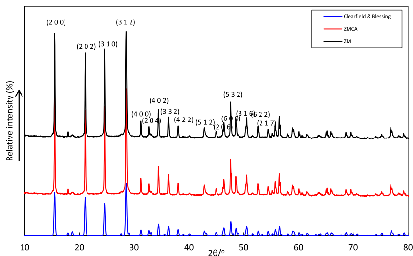
Fig. 16. X-ray diffraction pattern for zirconium molybdate, zirconium citratomolybdate and a comparison to zirconium molybdate particles synthesised by Clearfield and Blessing.
