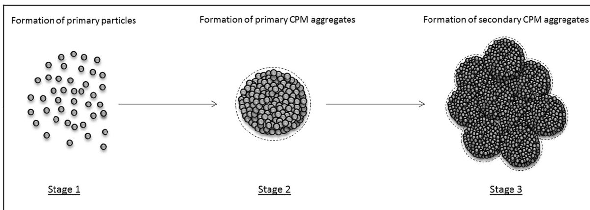
Fig. 6. Proposed aggregation mechanism for caesium phosphomolybdate particles. Stage 1: formation of the nanocrystallites; Stage 2: formation of the primary aggregates, consisting of cemented nanocrystallites; Stage 3: formation of the secondary aggregate, consisting of the submicron aggregates.
