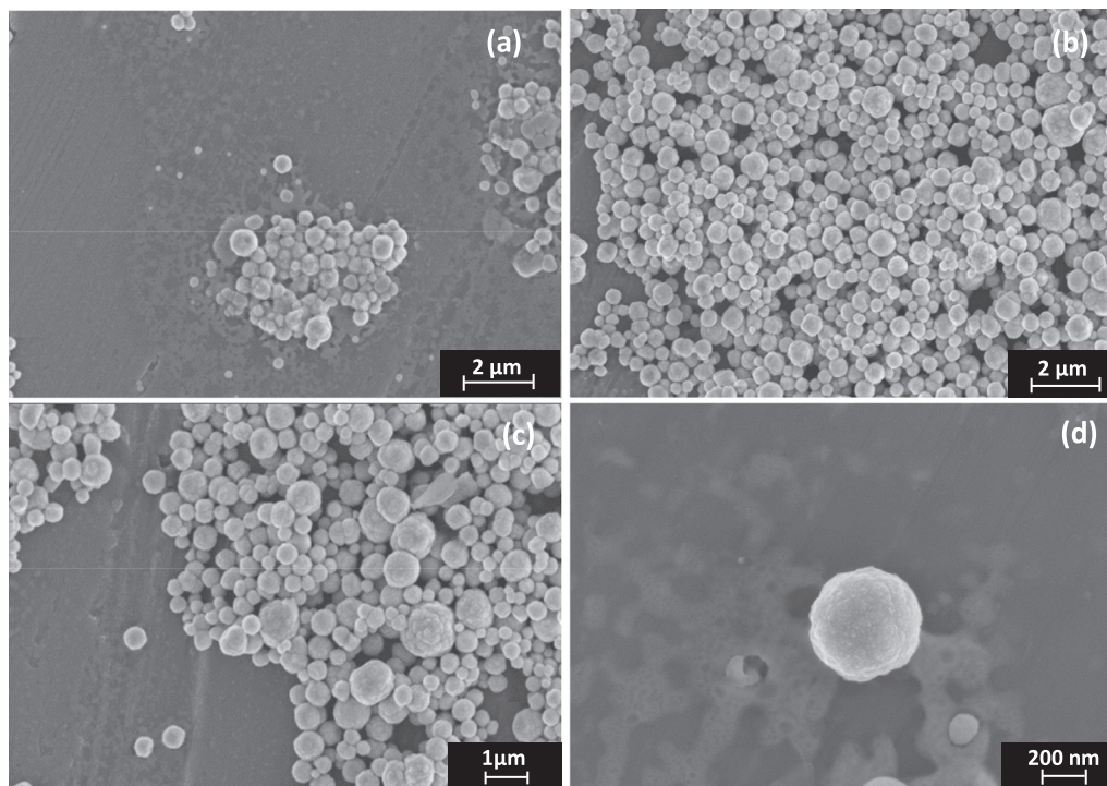
Fig. 5. Scanning electron microscope images of synthesised caesium phosphomolybdate particles. Images are taken at different magnifications: (a) 23.01 K; (b) 23.25 K; (c) 29.32 K; (d) 151.09 K.
