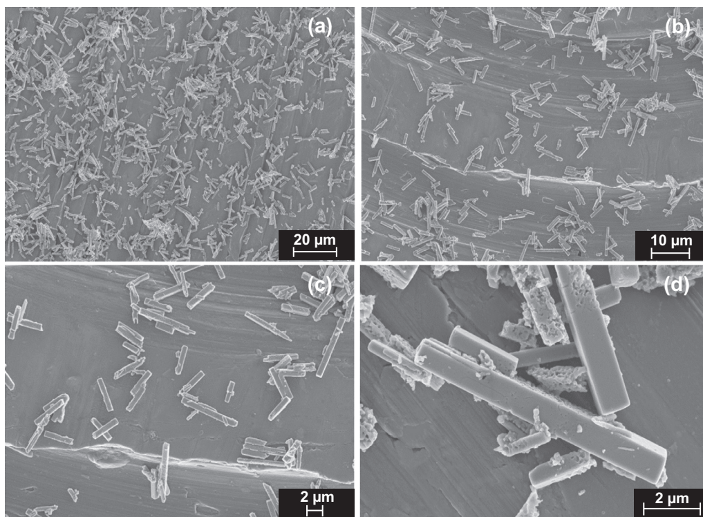
Fig. 14. Scanning electron microscope images of synthesised zirconium citratomolybdate particles. Images are taken at different magnifications: (a) 1.90 K; (b) 3.16 K; (c) 6.74 K; (d) 25.05 K.
