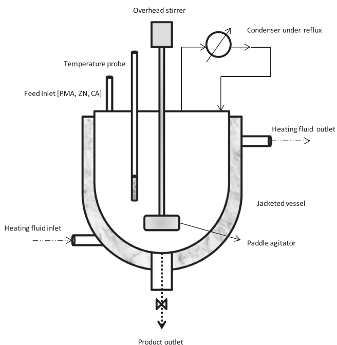
Fig. 1. A 4 L Batch reactor vessel set-up for caesium phosphomolybdate, zirconium molybdate and zirconium citratomolybdate synthesis. The reactor vessel is a jacketed vessel (containing silicon oil for heating purposes) an overhead paddle agitator, a condenser with circulating water at 5 °C and a temperature probe.
