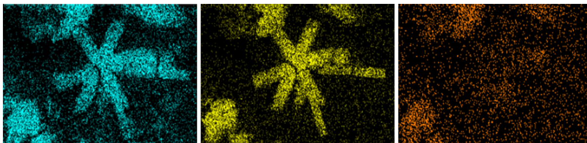
Fig. 13. Electron-dispersive X-ray images displaying elemental mapping of zirconium citratomolybdate at 336 h. Images taken for several elements: (a) Zr L \alpha 1; (b) Mo L \alpha 1; (c) Cs L \alpha 1.
