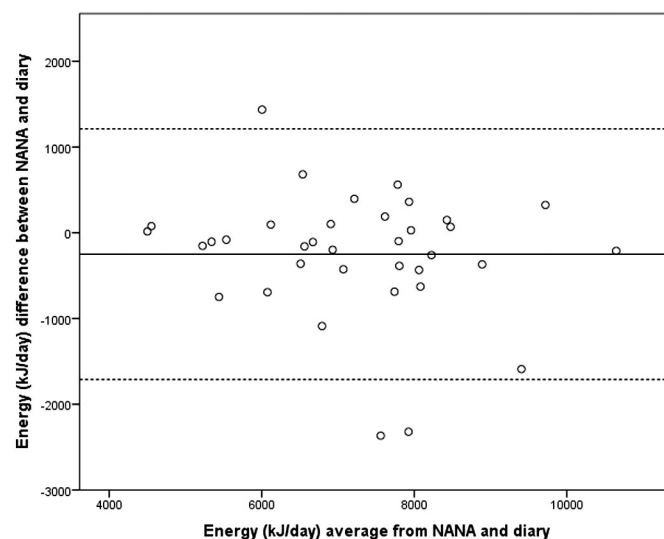
Fig. 3. Bland–Altman plot (NANA–food diary) of the difference between energy intake recorded by the NANA method with that recorded by the 4-day food diary against the mean energy intake for the 2 methods. Mean difference [solid line] and upper and lower limits of agreement (mean difference \pm 2SD) [dashed lines] for energy: -250 kJ/day, -1711/1212 kJ/day.
