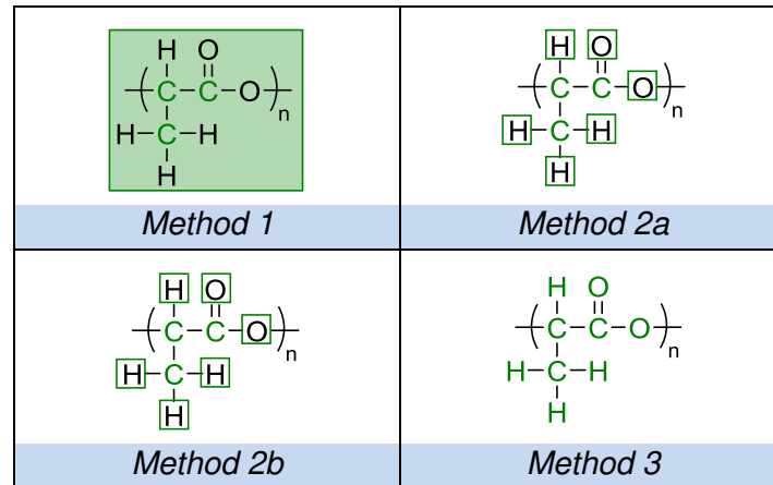
Figure 4-21 Atom allocation assignments for poly(lactic acid).
