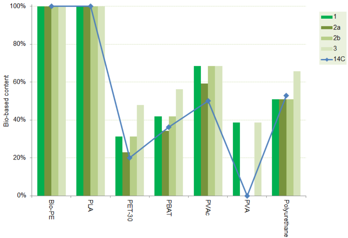
Figure 4-17 A summary of bio-based content atom connectivity method results for different bio-based plastics.
