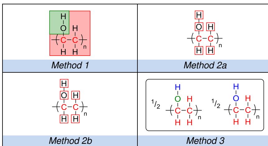
Figure 4-25 Atom allocation assignments for poly(vinyl alcohol).
