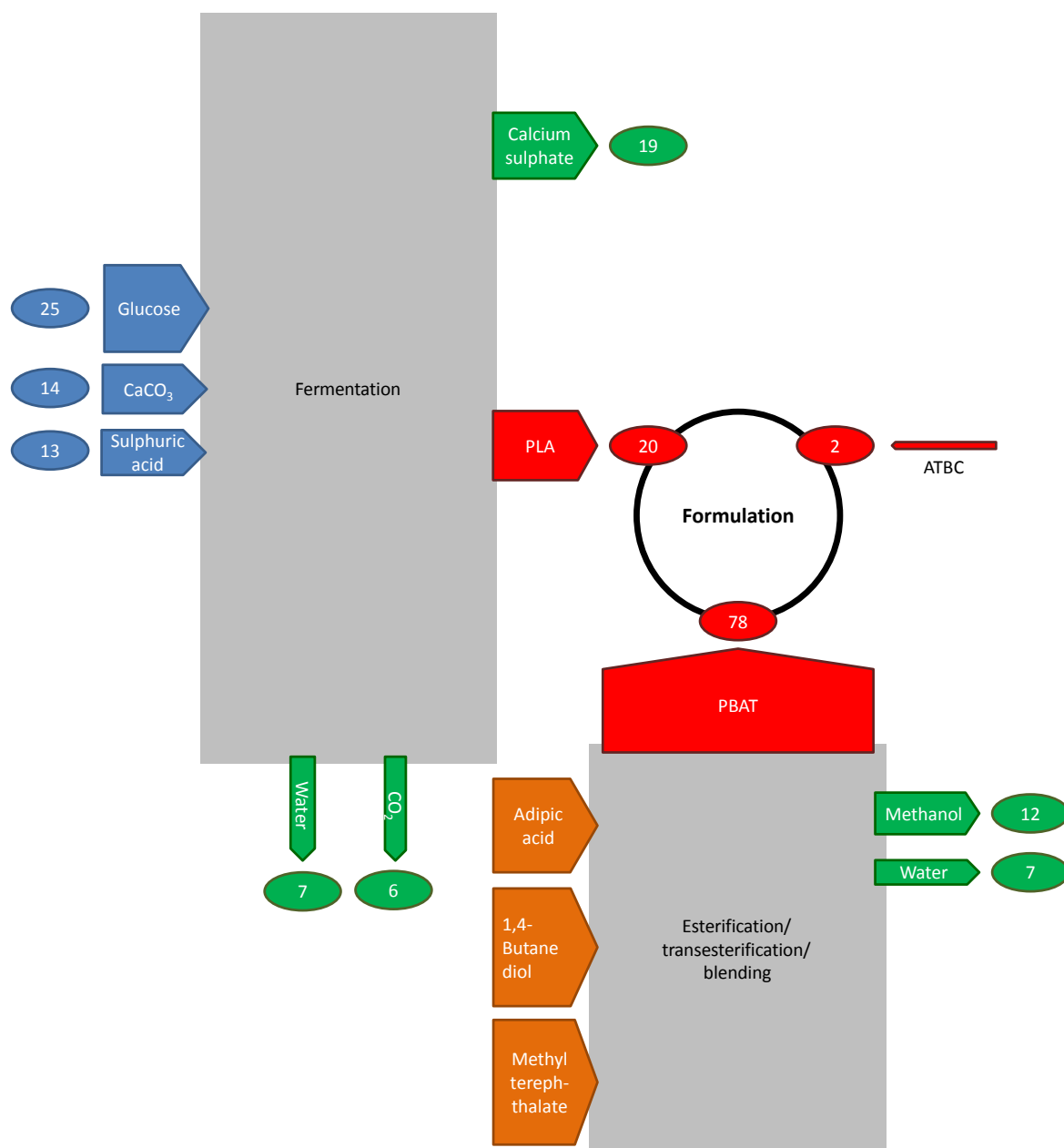
Figure 5-50 A Sankey diagram representing the production of poly(lactic acid) and subsequent formulation to produce a blend of poly(lactic acid) and poly(butylene adipate terephthalate) with a 1:4 mass ratio also containing acetyl tributyl citrate.
