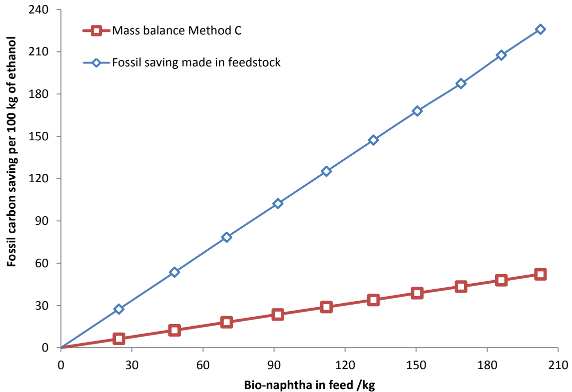
Figure 5-19 Fossil carbon savings based on the final product ethanol (in red) and the feedstock (in blue) per 100 kg of ethanol product manufactured according to mass balance Method C.
