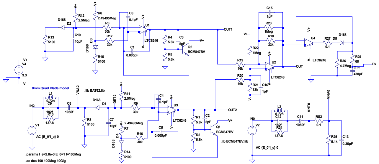
Figure 8. Log amplifier and detector final design including antenna model and linear detector/antenna model
