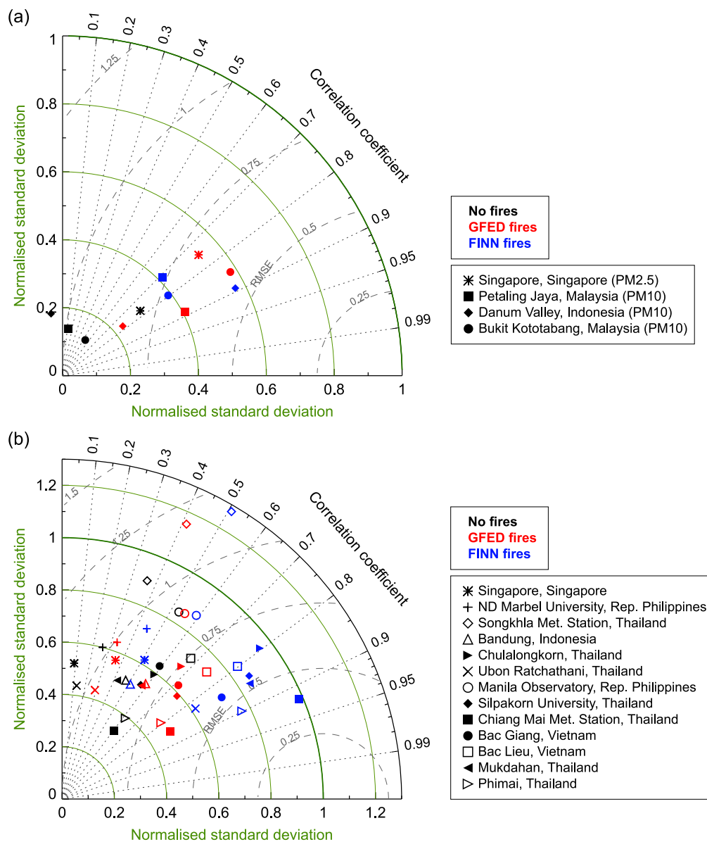
Figure 3. Taylor diagrams comparing monthly-mean modelled (GLOMAP) and observed (a) PM 2.5 and PM 10 at four aerosol measurement stations in Singapore, Malaysia and Indonesia; and (b) AOD (440 nm) at 13 AERONET stations located across Southeast Asia (locations shown in figure 1 and time periods in table S1). The modelled and observed monthly-mean AOD was calculated using daily means, with days corresponding to missing AERONET data removed prior to calculating the monthly-mean value. The observations are represented by a point on the x-axis at unit distance from the y-axis. Results are shown for three model simulations: (i) without fire emissions ('No fires'); (ii) with GFED3 fire emissions ('GFED'); (iii) with FINNv1 fire emissions ('FINN') (this simulation cannot be compared with PM 2.5 observations in Singapore because FINN emissions are not available for the year 2000). The model standard deviation and RMSE are normalized by dividing by the corresponding observed standard deviation. The normalized standard deviation and RMSE values are marked by the green-solid and grey-dashed lines respectively.
