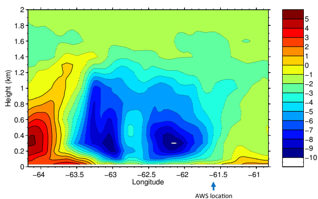
Figure 13. Vertical cross section through the straight black line in Fig. 8c for 15:00 UTC, 6 January. The colours show the component horizontal wind velocity ( \text{m s}^{-1} ) in a direction perpendicular to the line. Positive values indicate the component directed out of the page in an approximately northerly direction. The location of the AWS is also marked.
