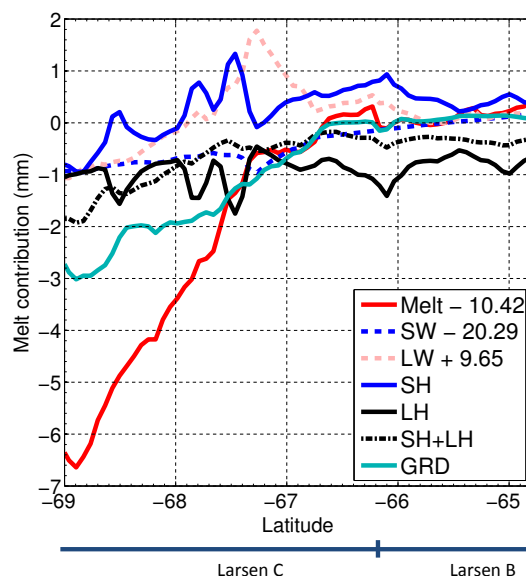
Figure 19. Simulated total melting amount averaged along lines of constant latitude across the Larsen ice shelf (“Melt”) for the times of 12:00, 15:00, 18:00 and 21:00 UTC, 6 January. Also shown are the net contributions to the surface melting (i.e. positive values indicate a net downward contribution) at these times from short-wave radiation (“SW”), long-wave radiation (“LW”), sensible heat flux (“SH”), latent heat flux (“LH”), combined sensible and latent heat flux (“SH + LH”) and ground heat flux (“GRD”). The lines “Melt”, “SW” and “LW” have been shifted by -19.8 , -27.7 and +7.6 mm respectively in order to make all the lines visible on the same plot. These shifts were designed to make the values zero at the Larsen B reference location at 65.6^\circ S. The approximate boundary between Larsen B and Larsen C is also marked.
