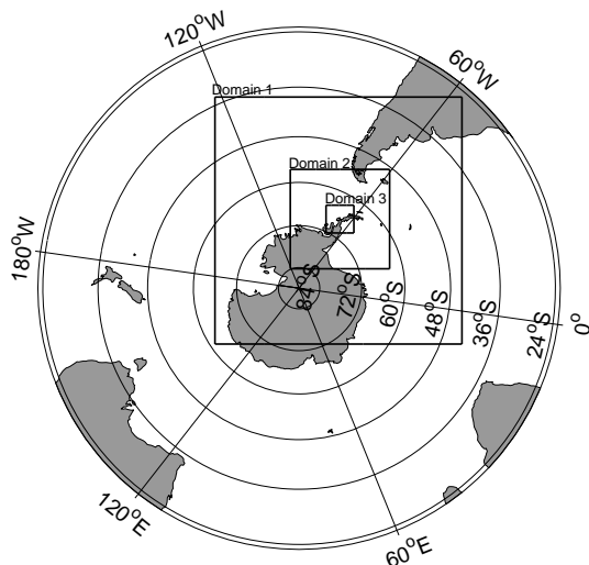
Figure 1. Locations of the WRF (Weather Research & Forecasting) model domains used in this study. The square domains had sides of length 7470, 3000 and 840 km with horizontal resolutions of 30, 7.5 and 1.875 km resolution for domains 1, 2 and 3, respectively.
