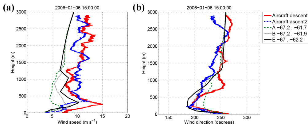
Figure 10. As for Fig. 5 except for at 15:00 UTC, 6 January and for wind speed (a) and direction (b) only. See Fig. 8c for a map of the locations of these profiles.
