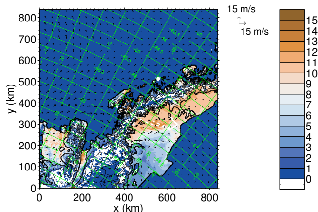
Figure 18. Total simulated snowmelt for domain 3 for the times of 12:00, 15:00, 18:00 and 21:00 UTC, 6 January in mm of water equivalent. The wind vectors are from the fourth model level taken at 12:00 UTC.
