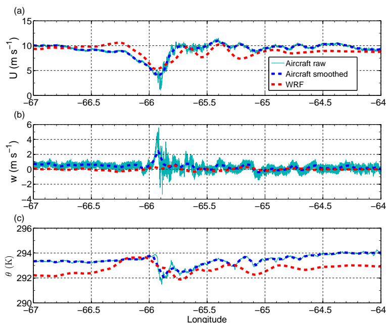
Figure 16. A comparison between the aircraft and WRF model at a height of 2900 m along similar west to east transects. For the WRF model, the transect is for 09:00 UTC, 6 January. For the aircraft the observations were made between 19:31 and 20:14 UTC, 6 January. The aircraft data has been binned into 2 km segments in order to match the horizontal resolution of the model (“Aircraft smoothed” on the legend). The original high-frequency data is shown as a thin line labelled “Aircraft raw”. Shown are (a) the component horizontal wind speed, (b) the vertical wind speed and (c) the potential temperature.
