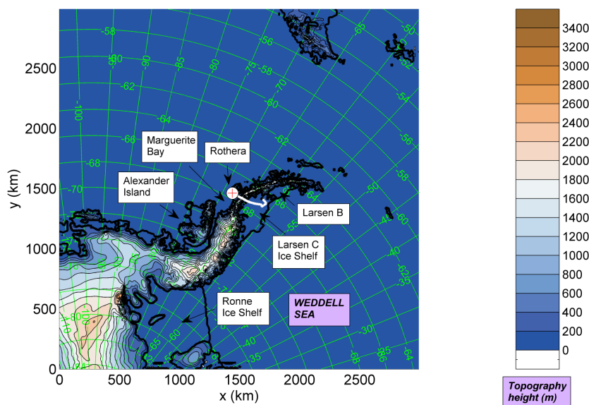
Figure 3. The area of the second WRF domain (see Fig. 1) showing the topography height (coloured contours) and various landmarks, including the Rothera BAS research base (white dot with red cross inside). The aircraft flight track is indicated by a white line.
