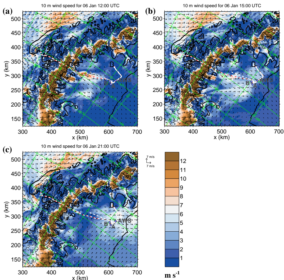
Figure 12. 10 m wind speeds (colours and vectors) for 6 January at (a) 12:00 UTC, (b) 15:00 UTC and (c) 21:00 UTC.
