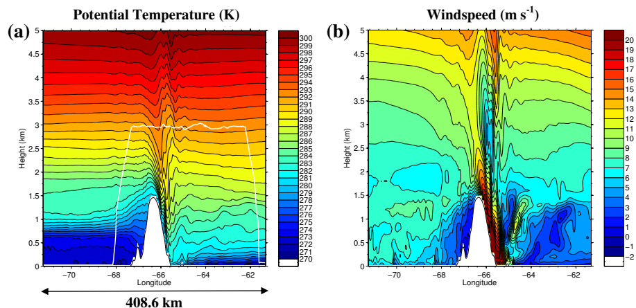
Figure 15. Vertical cross sections of potential temperature (a) and horizontal component wind speed (b) along the straight line in Fig. 8a for 09:00 UTC, 6 January. The white solid line in (a) shows the height of the aircraft projected onto the longitude of the cross section.
