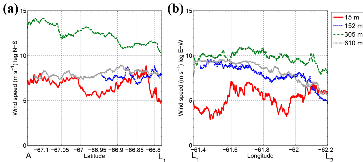
Figure A1. Wind speed during the “L” shaped legs flown from A to L1 to L2 at the heights indicated. See Fig. 8d for the position of these locations. The A–L1 leg was orientated close to south–north and the L1–L2 leg close to east–west. Thus, the x axis was chosen to be latitude for the A–L1 leg (a) and longitude for the L1–L2 leg (b). Also, here the data has been smoothed over 3 s windows for clarity. Note, part of the N–S leg at 152 m in (a) has been removed due to wind measurement problems caused by a loss of GPS lock.
