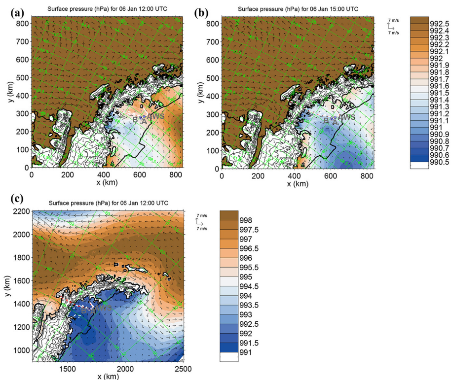
Figure 14. Surface pressure (colours; hPa) and 10 m wind vectors for 6 January. (a) and (b) show WRF domain 3 at 12:00 and 15:00 UTC, respectively, and (c) shows a close up of domain 2 at 12:00 UTC.
