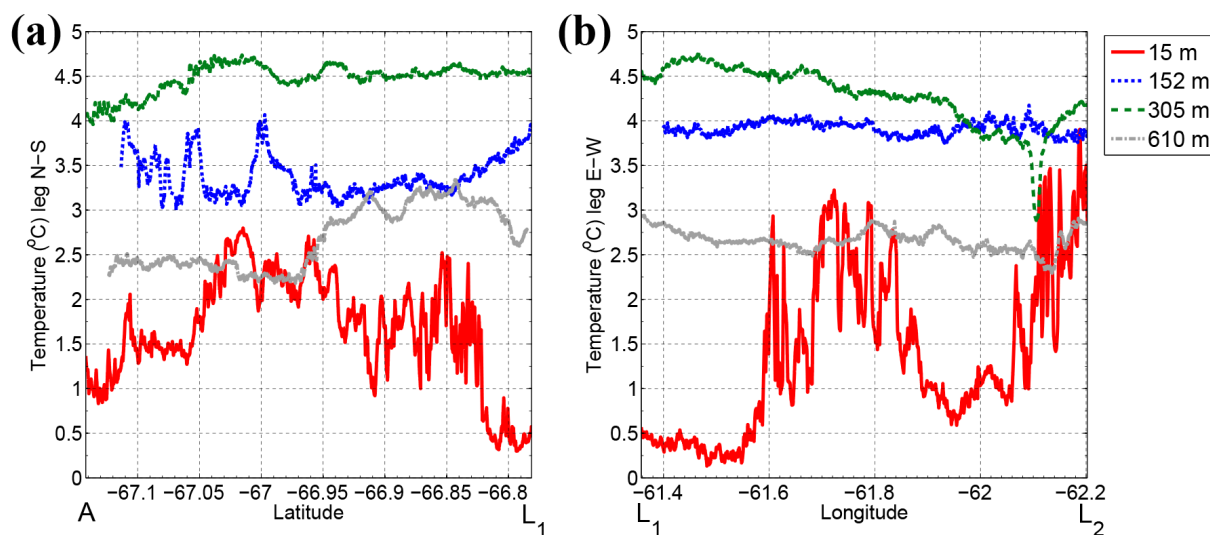
Figure A2. As for Fig. A1 except for temperature and with no smoothing.
