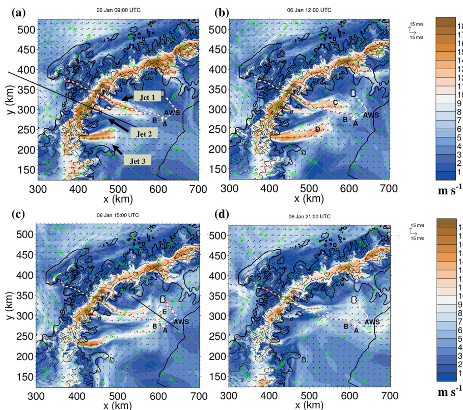
Figure 8. As for Fig. 6 except in close up view over the ice shelf and at different times on 6 January: 09:00 UTC (a), 12:00 UTC (b), 15:00 UTC (c) and 21:00 UTC (d). Also marked are the locations of various other points where the model profiles in Figs. 5 and 10 have been taken. The black straight line in (a) is the line over which the cross sections in Fig 15 were taken, and the line in (c) is that for the cross section in Fig 13.
