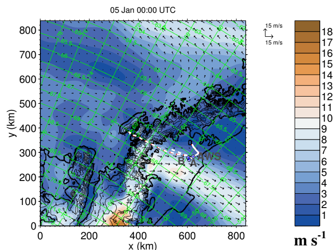
Figure 6. Domain 3 horizontal wind speed and wind vectors on the fourth vertical model level at the beginning of the simulation at 00:00 UTC, 5 January. This therefore represents the initial wind field as interpolated from the ECMWF analysis. Marked on here is the flight path of the aircraft (white dotted line). The marked location, A, is where the maximum wind speed was measured during the aircraft's descent onto the ice shelf. Location B is the position of the maximum wind speed during the ascent from the ice shelf before flying back over the peninsula. Also marked is the location of the automatic weather station (AWS).
