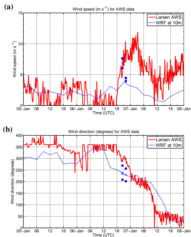
Figure 11. Time series from the Larsen C AWS along with the modelled values at the AWS location in domain 3; (a) 10 m wind speed ( S ) and (b) 10 m wind direction ( \phi ). Also marked are details of aircraft observations made during the A–L1 leg at 15 m altitude. For S the mean values are shown by the blue cross and the filled squares denote \pm 1\sigma . For \phi the squares denote the full range of the wind direction during the leg and the cross shows the midpoint of the range. The circles show the observed value when the aircraft was directly above the AWS location. The same is marked for the later descent towards the ice shelf just before the final ascent from the region.
