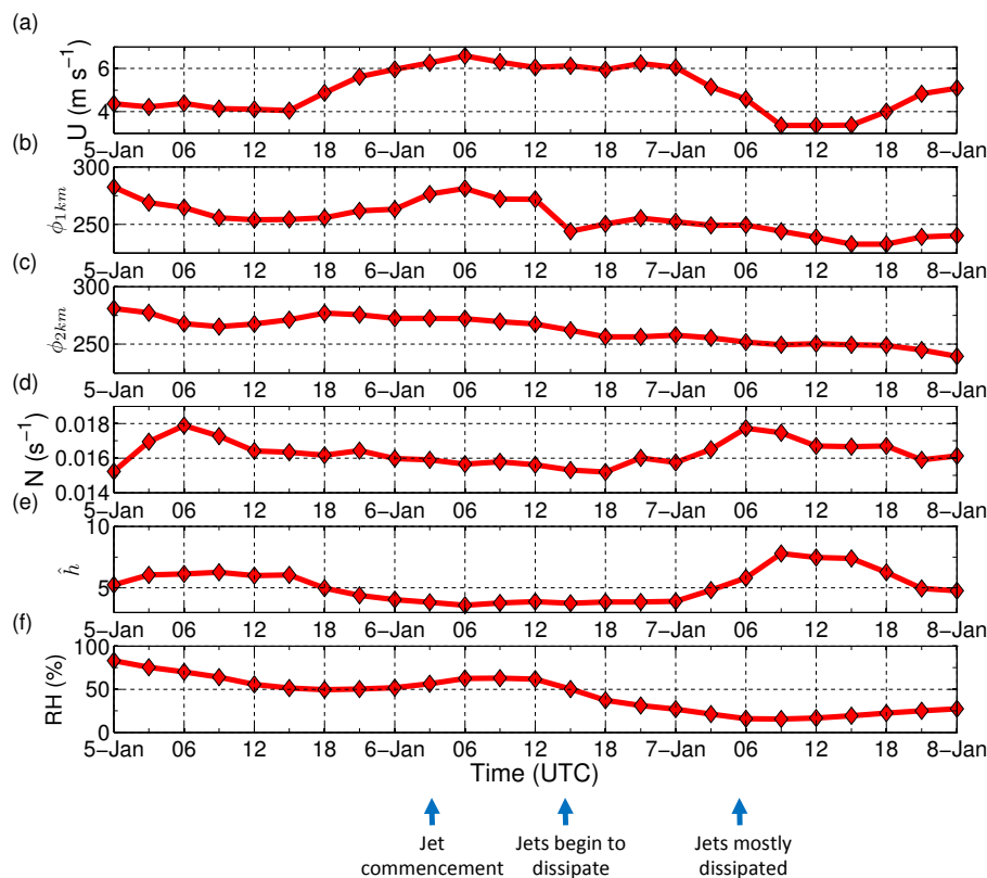
Figure 17. Time series of various quantities taken from the profile at the lefthand edge of the cross section in Fig. 15. (a) shows the component horizontal wind for the cross section averaged between heights of 0 and 2 km; (b) and (c) show the wind direction ( \phi ) at heights of 1 and 2 km, respectively; (d) shows that Brunt Väisälä frequency; (e) shows the non-dimensional mountain height; and (f) shows the relative humidity (RH) at a height of 2 km. Also marked are notable times for the development of the near-surface jet on Larsen C.
