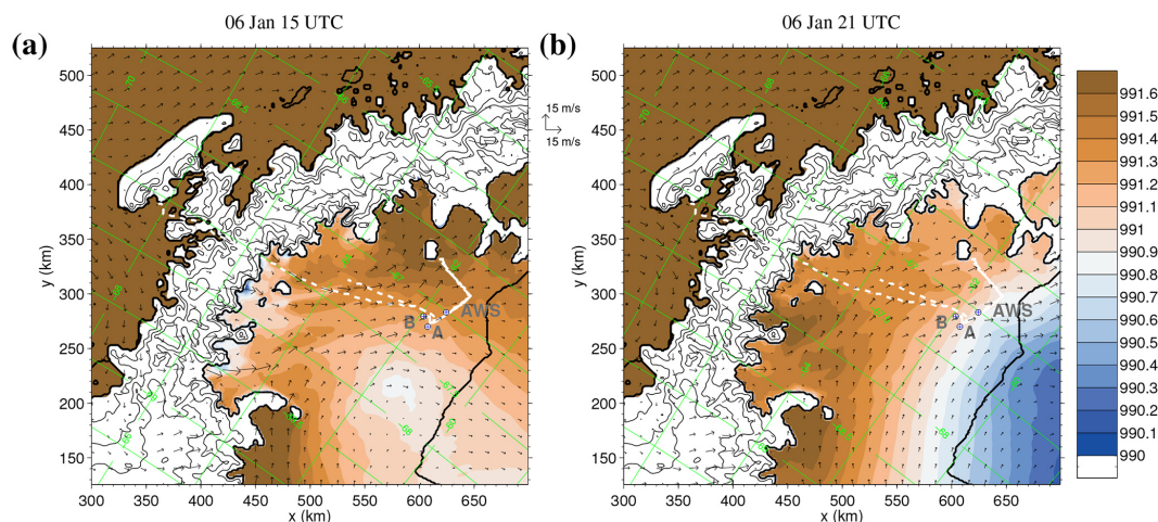
Figure 9. Surface pressure (colour contours; hPa) with wind vectors for the fourth model level at 15:00 UTC (a) and 21:00 UTC (b) 6 January.
