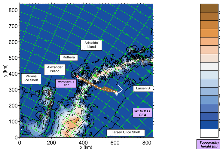
Figure 4. As for Fig. 3 except for the third WRF domain (see Fig. 1) and that here the black topography contours are every 500 m. The aircraft flight track is indicated by the white dotted line surrounded by coloured circles, which show the aircraft altitude on the same colour scale as the topography.
