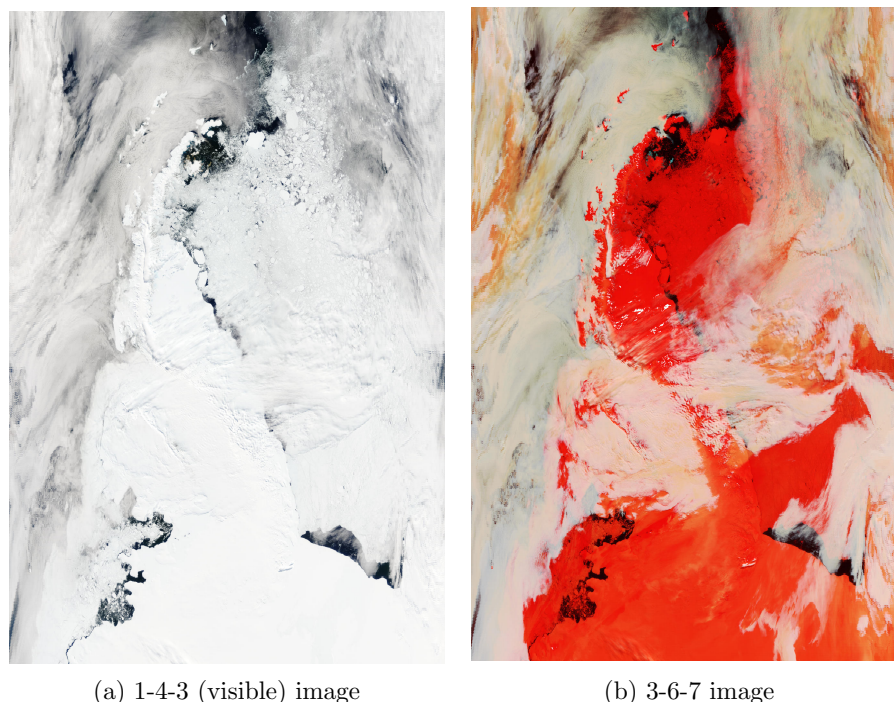
Figure 7. MODIS images over the Antarctic Peninsula region from 13:00 UTC, 6 January. (a) shows the visible image (bands 1, 4 and 3 used for red (R), green (G) and blue (B), respectively). (b) shows a false colour image using, respectively, bands 3, 6 and 7 for RGB. In (b) ice covered land shows up as red, whereas cloud shows up as white. The image is orientated approximately with north at the top and south at the bottom. The outline of the ice shelf, the ice covered land and sea ice to the east of the ice shelf can be discerned in (a) – see Fig. 4 to aid identification. (b) demonstrates that most of the Larsen C ice shelf was relatively cloud free. (a) shows that the cloud upwind (west) of the ridge is quite thin, whereas much thicker cloud is present along the ridge crest (except in the central portion of the ridge just north of Adelaide Island). Images were taken from http://lance-modis.eosdis.nasa.gov/cgi-bin/imagery/single.cgi?image=crefl1_143.A2006006130000-2006006130459.1km.jpg
