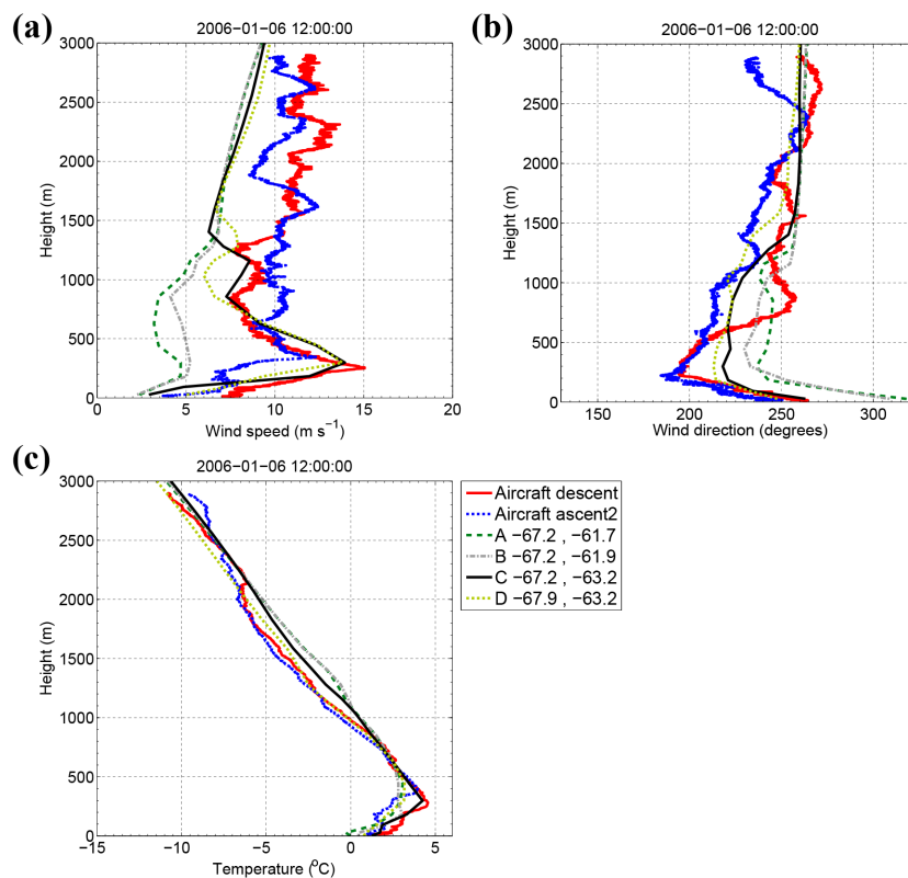
Figure 5. Profiles from the aircraft observations and from domain 3 of the WRF model. Aircraft profiles were taken during the descent down to the ice shelf between 20:14 and 20:24 UTC, 6 January and during the ascent away from the ice shelf before the journey back to base from 22:00 to 22:09 UTC. Model profiles are for 12:00 UTC, 6 January from various locations (labeled with letters in the legend). See Fig. 8b for a map of the locations of these profiles. The profiles are (a) wind speed, (b) wind direction and (c) temperature.
