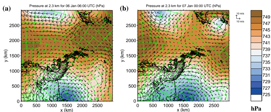
Figure 2. Pressure and wind vectors at 2.3 km a.s.l. for WRF domain 2 at (a) 06:00 UTC, 6 January and (b) 00:00 UTC, 7 January.
