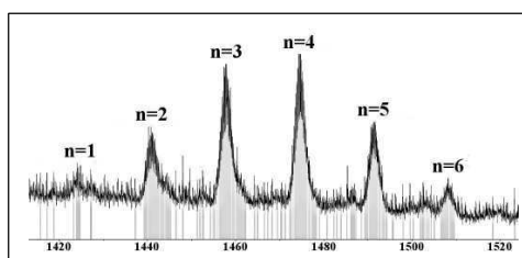
(i) ESI-MS of initial heteroleptic cage formation: \{[\text{Pd}_6(\mathbf{L1a})_{8-n}(\mathbf{L1})_n] \cdot 7\text{BF}_4\}^{5+}
