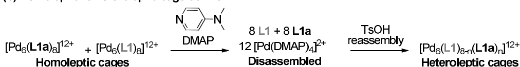
Scheme 3. Ligand speciation control of [\text{Pd}_6\text{L}_8]^{12+} stella octangula cages through (a) stoichiometry; (b) chemical disassembly and reassembly.
