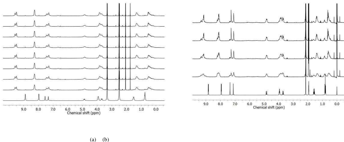
Figure 3. ^1\text{H} NMR spectra of ligand L1 (bottom trace) and the corresponding stella octangula complex [\text{Pd}_6(\text{L1})_8] \cdot 12\text{BF}_4 monitored over a week of standing the solution (a) [\text{D}_6]\text{DMSO} solution; (b) [\text{D}_3]\text{MeCN} (time increases on vertical scale).
