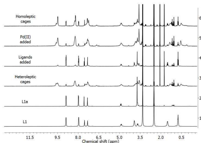
Figure 6. ^1\text{H} NMR of process (a) shown in Scheme 3. Speciation is changed from a mixture of heteroleptic cages to predominance of [\text{Pd}_6(\text{L1a})_8]^{12+} on addition of additional equivalents of both ligands, then to a mixture of homoleptic cages on addition of more [\text{Pd}(\text{MeCN})_4(\text{BF}_4)_2] (marked “Pd(II) added”). The top spectrum is a mixture of pre-formed homoleptic cages for comparison.
