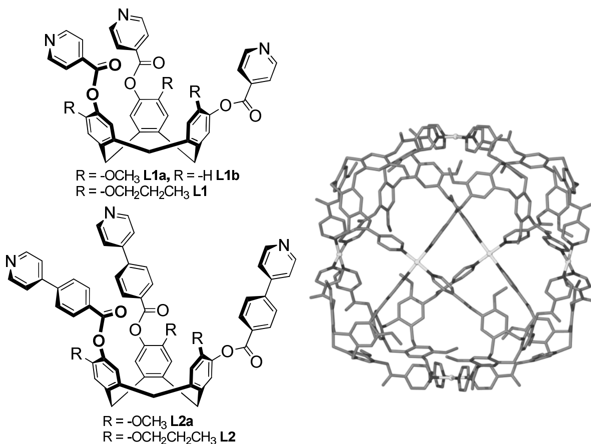
Scheme 1. Previously reported and target ( L1 , L2 ) pyramidal tripodal ligands with 4-pyridyl donor groups and the crystal structure of [Pd 6 ( L1a ) 8 ] 12+ from ref [9b].
