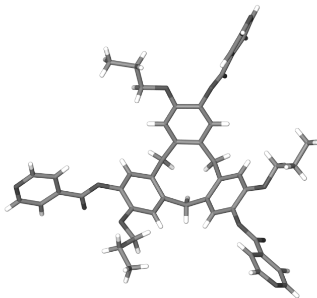
Figure 1. From the crystal structure of complex L1 ·0.5(MeNO 2 )·1.5(H 2 O).
