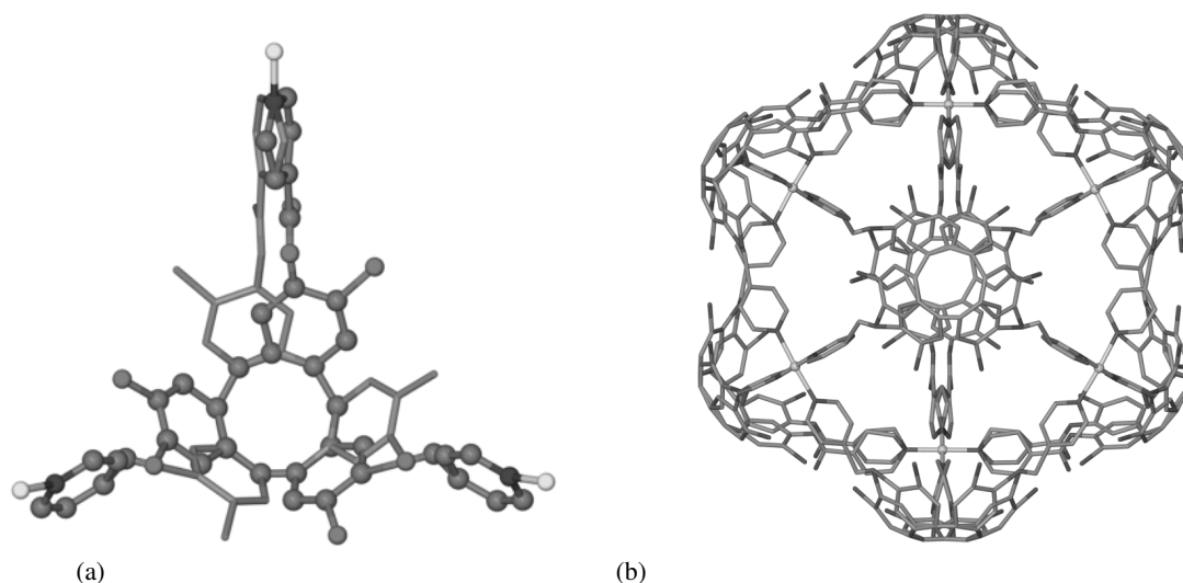
Figure 4. From the crystal structure of [\text{Pd}_6(\mathbf{L1})_8] \cdot 12(\text{BF}_4) \cdot 2(\text{H}_2\text{O}) . (a) Detail showing disordered ligand bridging between three \text{Pd}^{\text{II}} centres with the superposition of both ligand enantiomers, one enantiomer is shown in ball-and-stick to highlight; (b) the disordered [\text{Pd}_6(\mathbf{L1})_8]^{12+} stella octangula cage.
