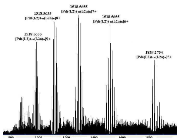
Figure 5. ESI-MS showing formation of heteroleptic [Pd 6 (L2) 8-n (L2a) n ] cages from a 4:4:6 mixture of L2:L2a:[Pd(MeCN) 4 (BF 4 ) 2 ]. Different charge states show different {[Pd 6 (L2) 8-n (L2a) n ] m (BF 4 ) 12-m+ series.
