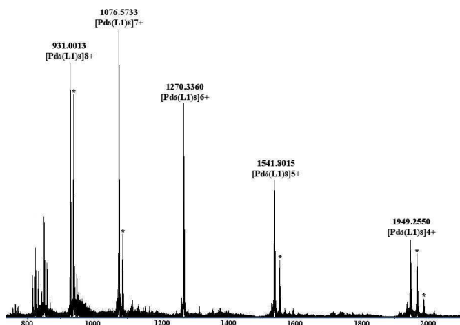
Figure 2. ESI-MS from mixture of L1 and [\text{Pd}(\text{MeCN})_4(\text{BF}_4)_2]_2 , showing various \{[\text{Pd}_6(\text{L1})_8] \cdot m(\text{BF}_4)\}^{12-m+} ions, asterisk indicate cage DMSO adducts.
