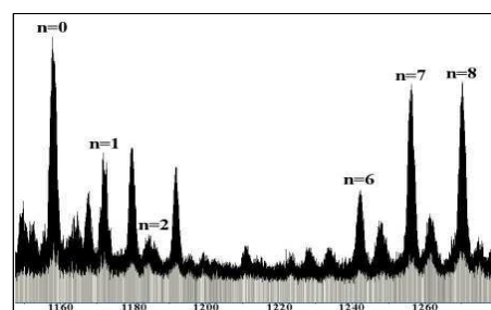
(ii) ESI-MS showing bias towards homoleptic cages: \{[\text{Pd}_6(\mathbf{L1a})_{8-n}(\mathbf{L1})_n] \cdot 6(\text{BF}_4)\}^{6+}
