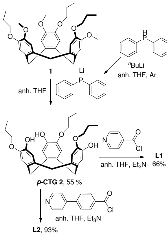
Scheme 2. Synthesis of the propylated CTG ligands L1 and L2 .
