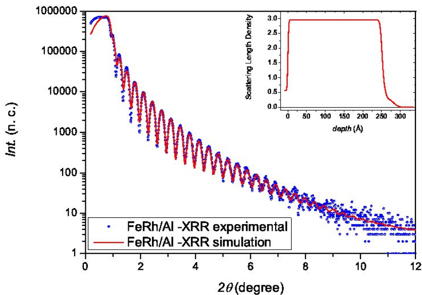
Figure 2. X-ray reflectometry spectrum from a 25 nm thick FeRh epilayer capped with polycrystalline Al. The solid line is a fit as described in the text, using the parameters given in Table 1. The inset shows the scattering length density profile associated with that set of fitting parameters. Click here to view larger figure
