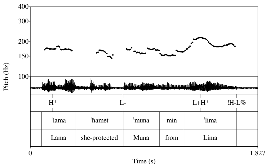
Fig. X.8 A downstepped plateau tune produced on the phrase /min 'lima/ “from Lima” as occurring in the utterance /'lama 'hamet 'muna min 'lima/ “Lama protected Muna from Lima”.
