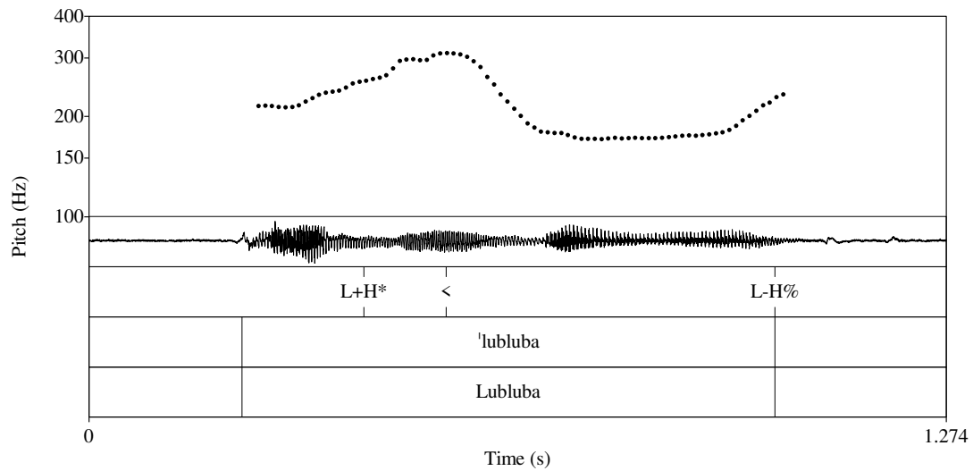
Fig. X.7 A stylized continuation tune produced on the proper noun /'lubluba/. The '<' symbol represents peak delay.
