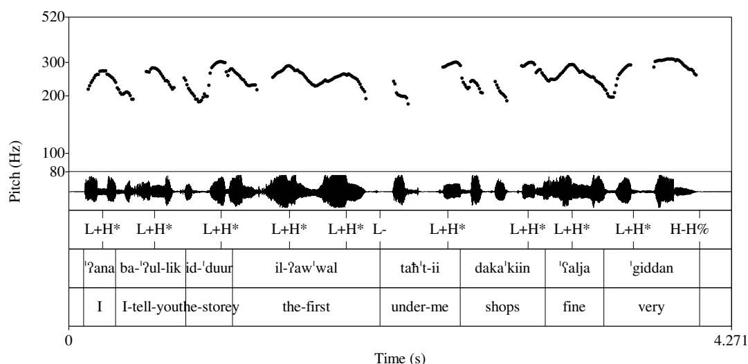
Fig. X.23 An example of secondary accents for pragmatic function on the word /lʔawwal/ in: [lʔana ba-lʔullik id-du:r il-lʔawwal.. taħ'ti: daka'ki:n lʔalja l'giddan] ‘I tell you the first ... below me (i.e. below my first floor apartment) there are really great shops’ (4862B: 483.25-487.40).
