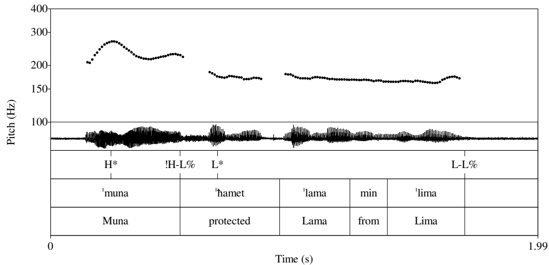
Fig. X.20 An example of phrasing and gradient pitch range manipulation in /'muna 'hamet 'lama min 'lima/ “Muna protected Lama from Lima”, with narrow focus on the utterance-initial target word.
