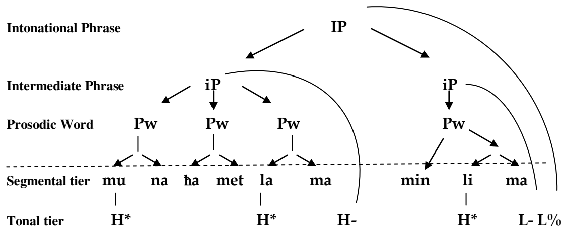
Fig. X.1 A metrical representation of the prosodic hierarchy in LA, illustrated for the utterance /'muna ʰamet 'lama min 'lima/ “Muna protected Lama from Lima”. This utterance is produced as two iP within a single IP. In the first iP /muna/ and /lama/ are pitch accented, in the second /lima/ is accented. The intonational structure of the utterance is: H* H* H- H* L-L%.
