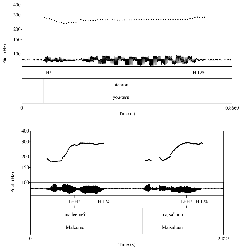
Fig. X.6 Typical plateau contours a) indicating incompleteness and produced on the word /btebrom/ “you turn”, and b) illustrating calling tunes produced on the proper nouns /ma'leemeʔ/ and /majsaluun/.
