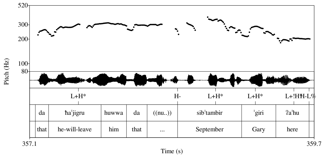
Fig. X.17 Example of H-L% open-ended boundary tone combination: [da ħa'jigru huwwa da... sib'tambir 'giri ?a'hu] “that one he will leave.. Gary will be here in September” (4862B 357.15-359.71).
