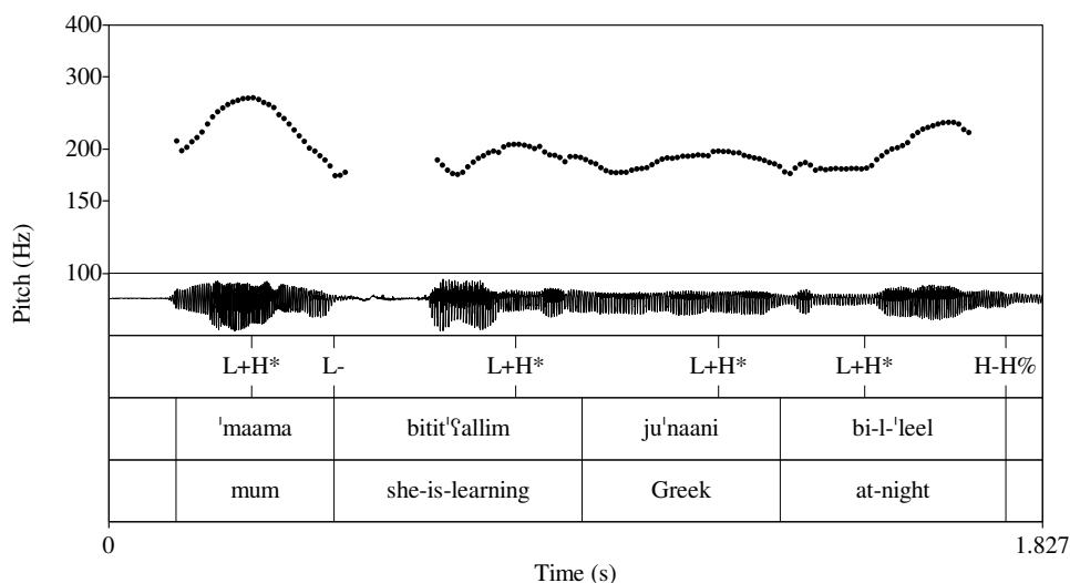
Fig. X.21 A read speech SVO sentence elicited with narrow contrastive focus on the subject [ˈma:ma], and such that the object [juˈna:ni] was old information, in: [ˈma:ma bititʔallim juˈna:ni bi-l-ˈle:l] “Mum is learning Greek in the evenings” (from Hellmuth 2006b).
