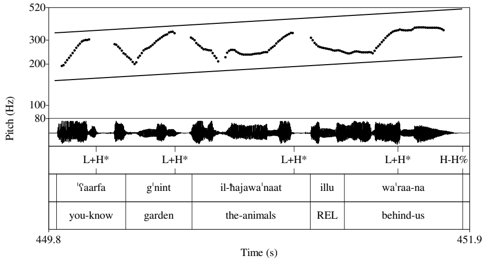
Fig. X.15 Spontaneous speech declarative question showing rising pitch register and a rising final boundary: [ʕa:rfa g'nint il-ħajawa'na:t illu wa'ra:na] “Do you know the zoo behind us (i.e. behind our house)?” (4682B 449.77-451.95). Register lines are schematic.
