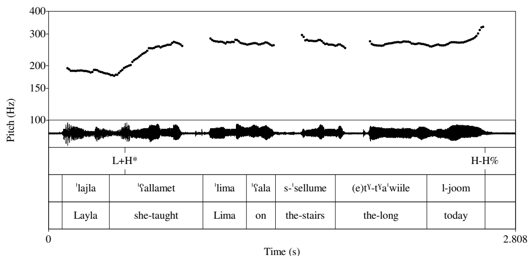
Fig. X.4 An illustration of LA YNQ tunes with a) a low nuclear accent on /'ɣindak/ “you have” in the utterance /'ɣindak 'jee/ “Do you have it?”, and b) a rising nuclear accent on /'ɣallamet/ “teach” in the utterance /'lajla 'ɣallamet 'lima 'ɣala 's-sellume tʰ-tʰa'wiile l-joom/ “Did Layla teach Lima on the stairwell today?”.
