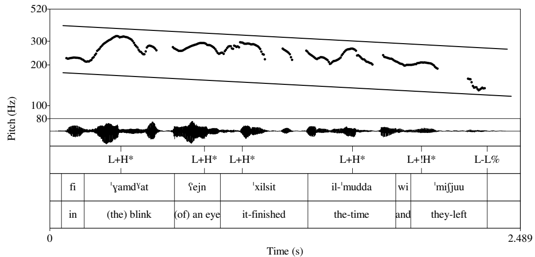
Fig. X.12 Spontaneous speech declarative showing declination and final lowering: [fi 'yamɖat ʔejn 'xilsit il-'mudda wi 'miʃju:] “in the blink of an eye they were gone” (4862A 364.61-367.05). Register lines are schematic only.
