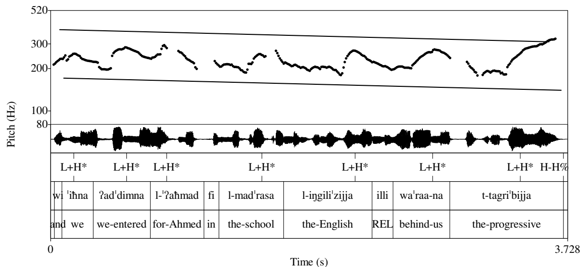
Fig. X.13 Spontaneous speech declarative showing a continuation rise: [wi 'iħna ʔad'dimna l-'ʔaħmad fi l-mad'rasa l-ʔiŋgili'zija illi wa'ra:na t-tagri'bija] “and we have entered Ahmed for the English school that’s right behind us” (4682B 330.53-334.27). Register lines are schematic only.
