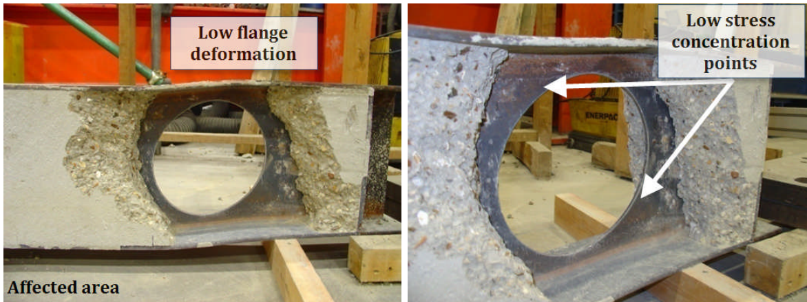
Fig. 18: Failure mode for partially encased USFB No.2 at opening after removal of the damaged concrete
