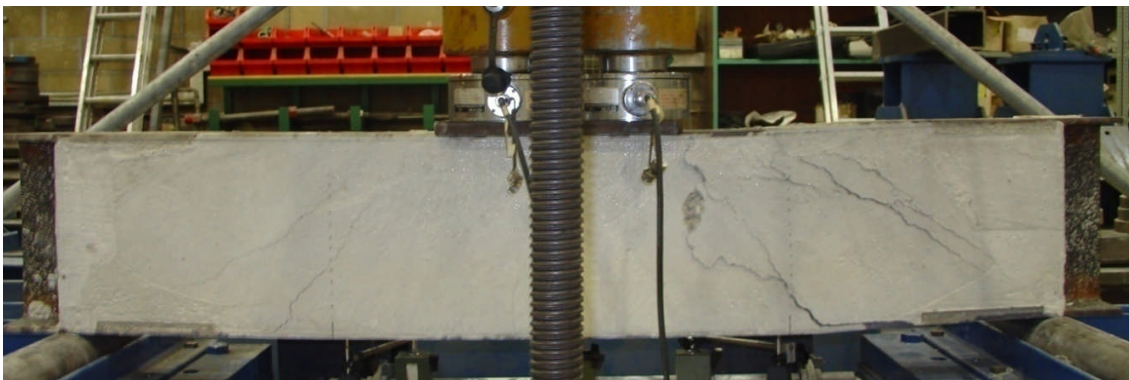
Fig. 11: USFB No.2 (concrete crushing)
