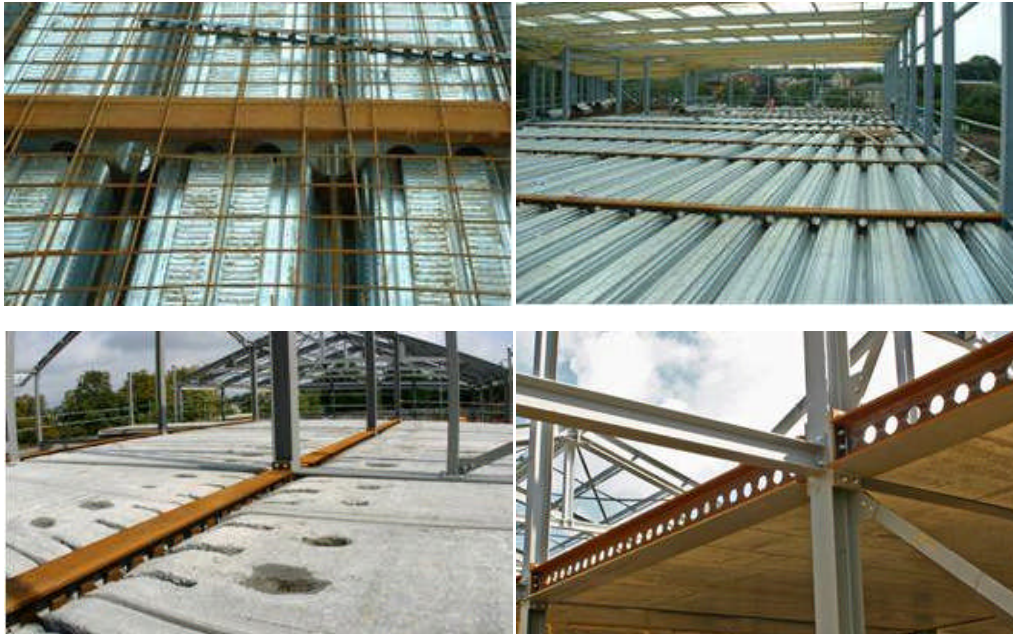
Fig. 1: USFB used with profiled steel decking (top) and with precast concrete unit (bottom) (adopted by [17])
