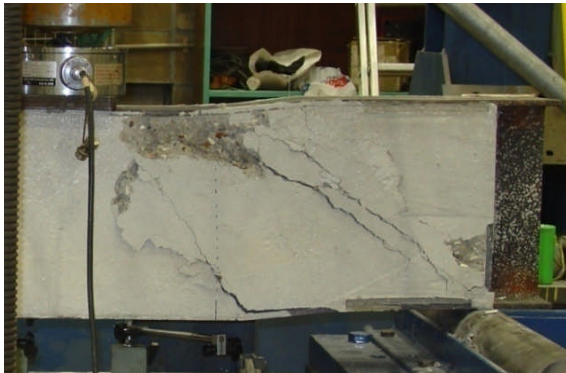
Fig. 14: USFB No.2 (concrete bursting)
