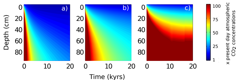
Fig. 8. Evolution of \text{CO}_2 profiles over 20 ka of soil development for three different model scenarios. N_p = 0.5 \text{ kg m}^{-2} \text{ yr}^{-1} and z_r = 0.26 (a) , N_p = 1 \text{ kg m}^{-2} \text{ yr}^{-1} and z_r = 0.26 (b) and N_p = 1 \text{ kg m}^{-2} \text{ yr}^{-1} and z_r = 0.5 (c) .
