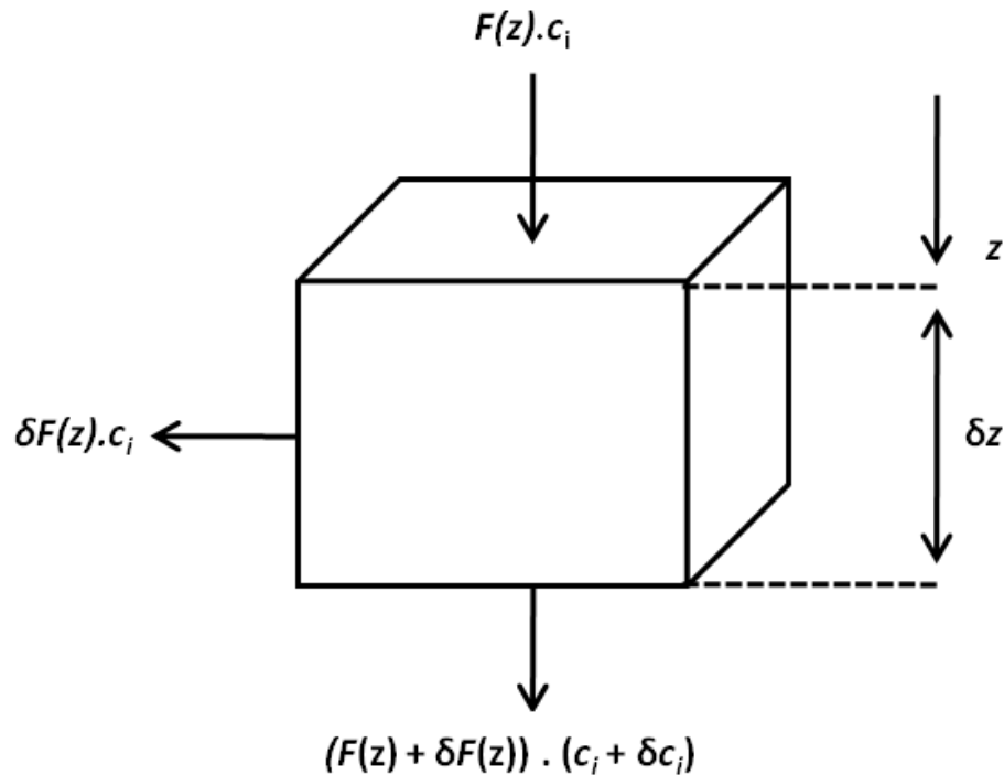
Fig. 1. Schematic overview of solute mass balance where F is the rate of percolation ( \text{myr}^{-1} ) at depth z and c is the concentration of ion i in solution ( \text{gm}^{-3} ). Adapted from Kirkby (1985)
