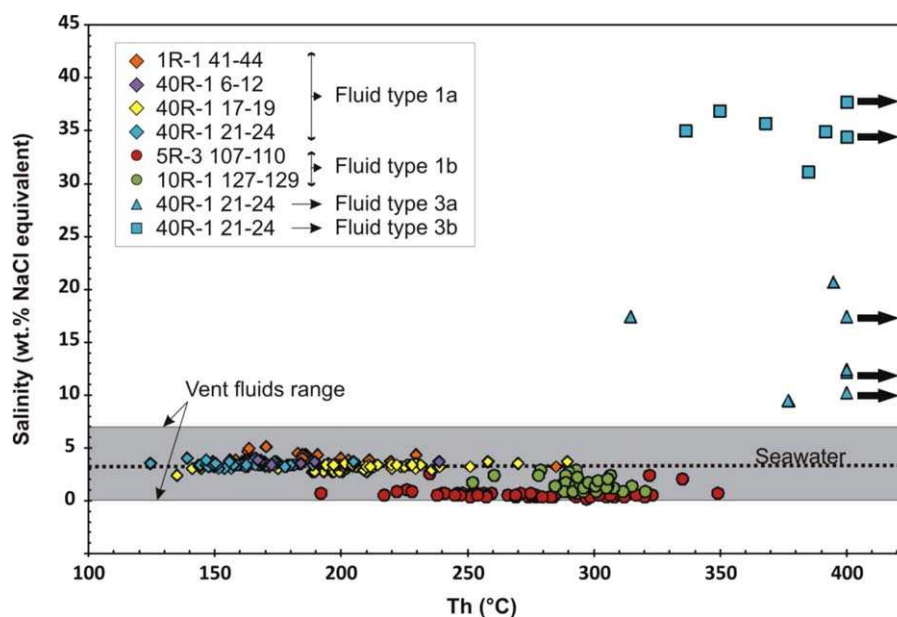
Figure 5. Temperature of homogenization against salinity for all samples. The shaded area represents the range in salinity for fluids exiting submarine hydrothermal vents. Arrows mean that fluid inclusions were not homogenized at this temperature (high temperature limit of apparatus).
