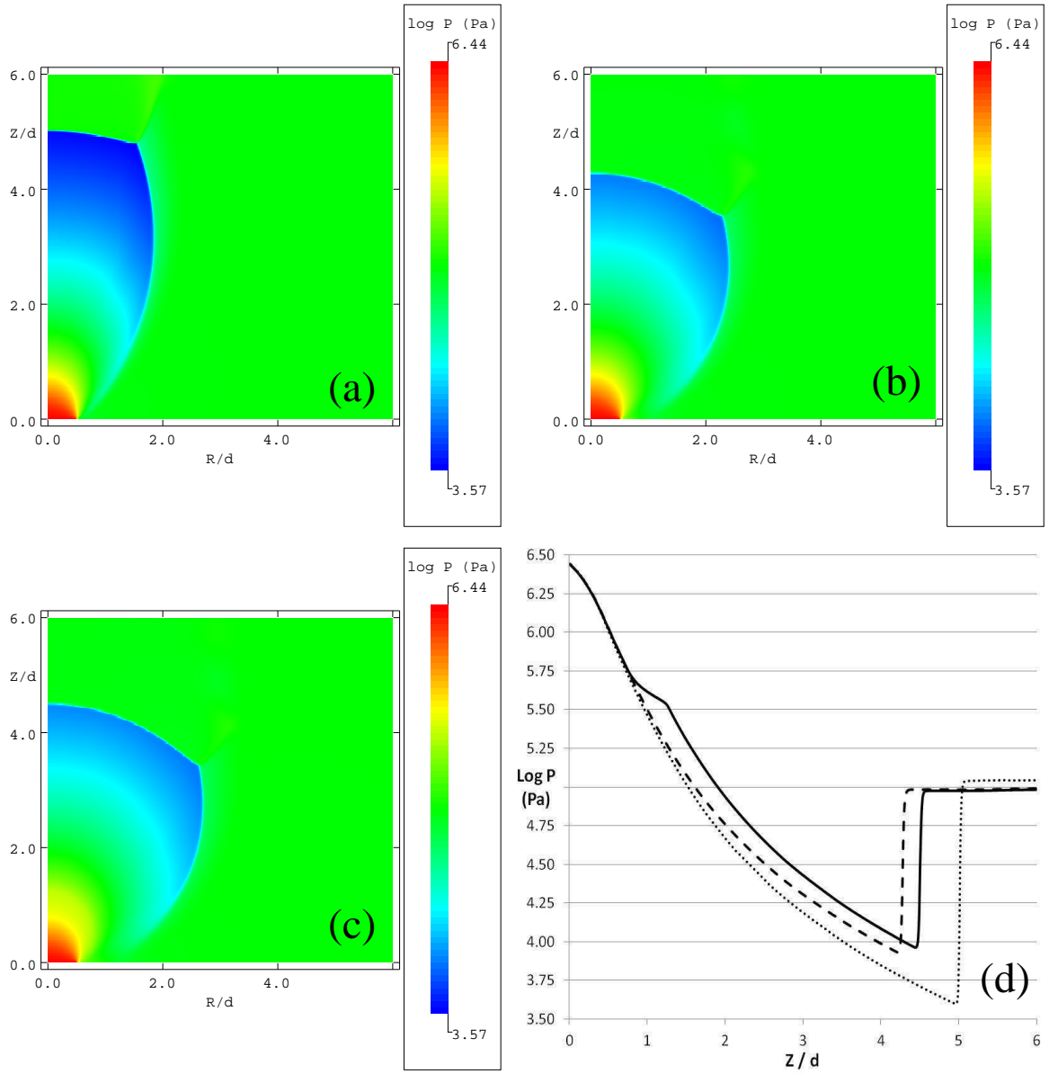
FIG. 10. Pressure in the near-field of the flow domain. This figure shows the pressure in the jet predicted by the ideal equation of state (a), the Peng-Robinson equation of state (b) and the composite equation of state (c). In panel (d), we show a comparison along the jet axis between the three models - ideal (dotted line), Peng-Robinson (dashed line) and composite (solid line).
