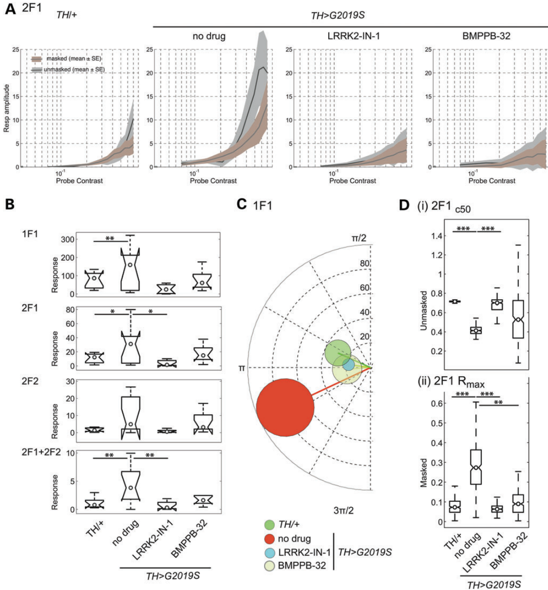
Figure 8. Kinase inhibitors targeted at LRRK2 restore normal responses in the presence of TH>G2019S at day 1. Data from four phenotypes are displayed: control ( TH+ ), untreated TH>G2019S and TH>G2019S flies raised on food containing kinase inhibitor drugs LRRK2-IN-1 or BMPPB-32 at 2.5 \mu\text{M} concentrations. (A) Contrast response functions for 2F1 show the increased signalling in TH>G2019S is reverted by LRRK2-IN-1 or BMPPB-32. (B) Average responses and data spread measured at a single contrast and mask level for different frequency components. The 1F1 signals derive primarily from the photoreceptor responses and are evaluated at 63% probe contrast. 2F1 signals are transient neuronal responses to the same input. 2F2 components derive from neuronal responses to the mask in the presence of a very weak probe input (30% mask contrast, 7% probe contrast). The 2F1 + 2F2 intermodulation term is likely to arise from non-linear interactions in deeper neuronal structures—here we evaluate it at its peak, which occurs when the probe and mask contrasts are approximately equal (probe = 35% contrast, mask = 30% contrast). At 1F1, 2F1 and 2F1 + 2F2, the presence of the hLRRK2-G2019S transgene elevates the response amplitude significantly ( P < 0.05 , Table 1). Responses from animals raised on 2.5 \mu\text{M} LRRK2-IN-1 are restored and statistically indistinguishable from those of the controls. The compound BMPPB-32 at 2.5 \mu\text{M} concentration also reduced the response amplitude at these frequencies, although the reduction only reached statistical significance in the intermodulation term (2F1 + 2F2). The responses of G2019S flies are notably more variable across individuals than those of the other organisms. (C) Phase plots for unmasked 1F1, showing that both LRRK2-IN-1 and BMPPB-32 restore control-level neuronal SSVEP responses phases measured at 63% probe contrast. Error circles are computed on the complex data using the t-circ statistic. (D) Estimated c_{50} values for each of the four phenotypes in (A), showing that the c_{50} value for TH>G2019S is approximately half that of the wild-type outcross ( TH+ ). Both kinase inhibitors restore the wild-type value. Statistical tests for the data shown in (B–D) are shown in Table 1. (In B and D, the plots show mean, 95% confidence intervals and data range. n = 10, 11, 12, 10 .)
