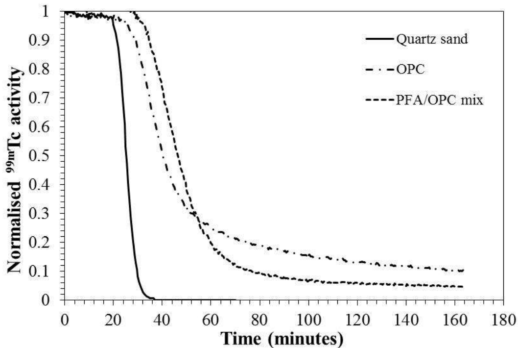
Figure 2. Total measured activity of ^{99m}\text{Tc} (normalised to input activity) as a function of time during transport through quartz sand, Ordinary Portland Cement (OPC) and OPC mixed with pulverised fly ash (PFA).
