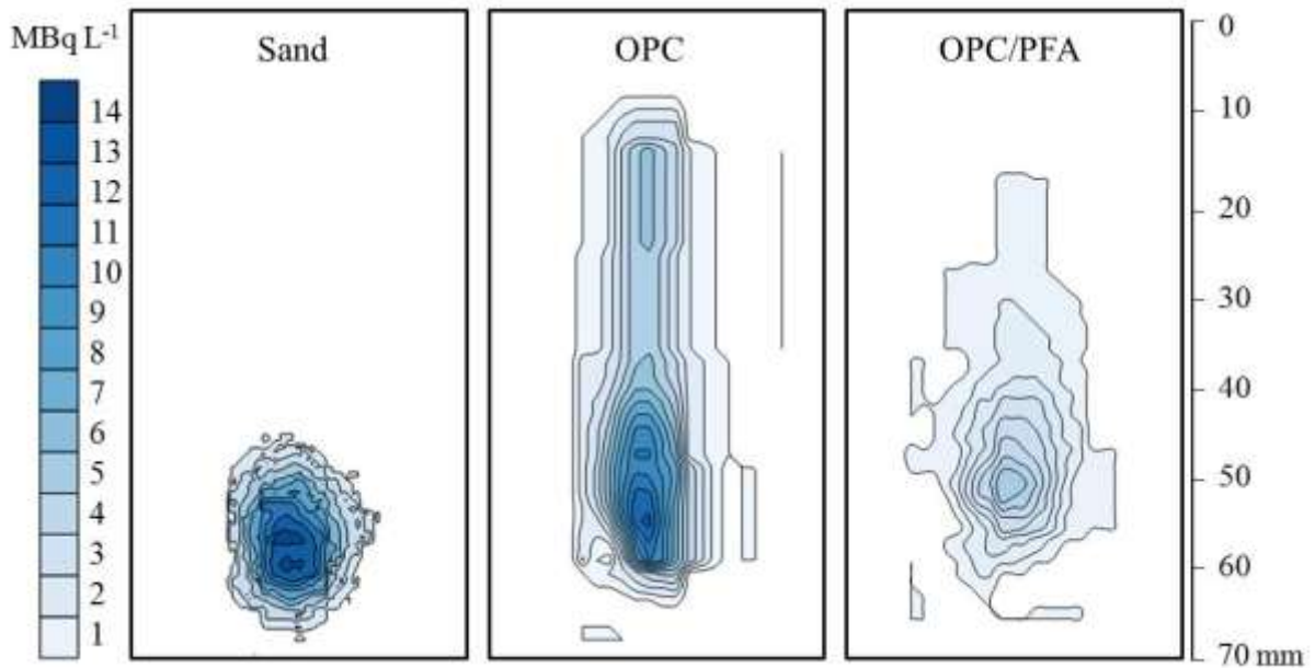
Figure 3. Calibrated concentration distributions derived from gamma camera images of ^{99m}\text{Tc} activity in quartz sand, Ordinary Portland Cement (OPC) and OPC mixed with pulverised fly ash (PFA) at 40 minutes after the injection of ^{99m}\text{Tc} .
