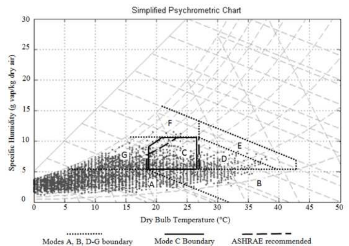
Figure 1 Psychrometric chart with weather data for Redmond, Oregon and the cooling system modes A to G for the data centre as per information from (Jay Park, 2011, Open Compute Project: Data Center v1.0). Also shown is the ASHRAE recommended envelope
