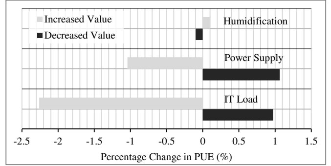
Figure 3 Percentage changes in PUE as a result of altering different parameters within the metric: (i) humidification by \pm 20\% , (ii) \eta_E by \pm 1\% , (iii) IT load by -40\% and +20\%
