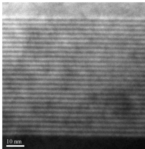
FIG. 5. TEM image of the graded barrier showing the layer separation in the “digital alloyed” graded barrier. A clear layer separation between GaAs and AlAs layers are visible in the structure except for the topmost region of the barrier, where a finer mesh digital grading was used.
