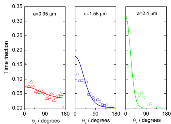
Figure 8. Scatter graphs showing the actual azimuthal angle, \theta_a , derived by resolving the measured propulsion and sedimentation velocity vectors. Solid line is P(\theta_a) estimated from a Boltzmann distribution for the gravitational energy cost for rotating a solid ellipsoid overlayer of platinum.
