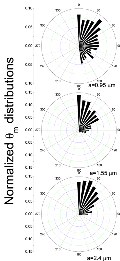
Figure 7. Normalized angle distribution for \theta_m as a function of radius for all translational steps for each recorded 2D swimmer trajectory.
