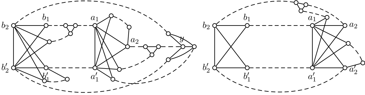
Figure 17: Paths from Lemma A.14.
