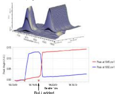
Figure 2. In situ IR 3-D and 2-D plots of the lithiation of 5 with n -BuLi at -50 °C in THF. Blue line represents intensity of C=O stretching frequency of 5 (1692 cm -1 ) and red line of lithiated 5 (1645 cm -1 ) over time (in min).
