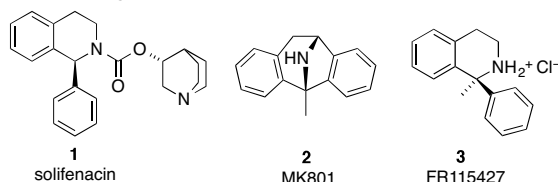
Figure 1. Some hydrogenated isoquinoline drugs.
