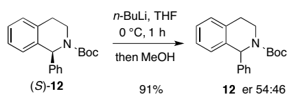
Scheme 7. Racemization of (S)- 12 (er 99:1).
