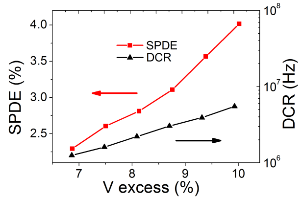
Fig. 5. SPDE and DCR as a function of excess bias for a 25- \mu\text{m} -diameter device at 100 K when measured at \lambda = 1310 nm.
