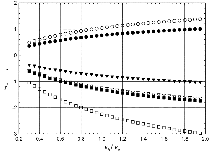
Fig. 3. \gamma^* versus v_h/v_e for (circles) \alpha w = 0.5 , (triangles) 1.0, and (squares) 2.0, for the constant (filled) and enhanced velocity (open) models. \beta = \alpha and d_e w = 0.1 = d_h w in all cases.
