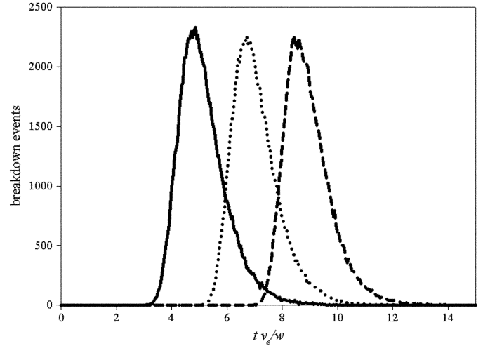
Fig. 5. RPL calculations of distributions of times to reach avalanche currents of (full line) 0.01 mA, (dotted line) 0.1 mA, and (dashed line) 1 mA assuming d_e/w = 0.1 with \alpha w = 2.5 and identical ionization parameters for electrons and holes.
