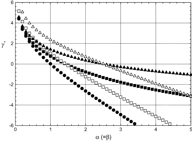
Fig. 1. \gamma^* versus \alpha w for d_e/w = 0 (circles), 0.1 (squares), and 0.2 (triangles), for the constant (filled) and enhanced velocity (open) models. v_e = v_h , d_e = d_h , and \alpha = \beta in all cases. The constant and enhanced velocity models coincide at d_e = 0 = d_h , as do their results.
