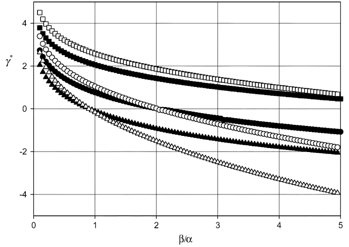
Fig. 2. \gamma^* versus \beta/\alpha for \alpha w = 0.5 (squares), 1.0 (circles), and 1.5 (triangles), for the constant (filled) and enhanced velocity (open) models. v_e = v_h and d_e w = 0.1 = d_h w in all cases.
