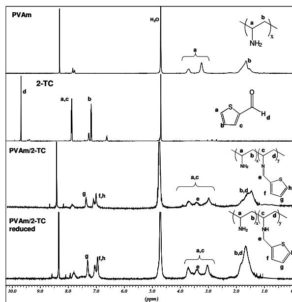
Fig.3 1 H NMR spectra (D 2 O) illustrating the chemical modification of poly(vinyl amine) (PVAm) via Michael addition with 10 mol % 2-thiophenecarboxaldehyde, 2-Tc: (a) poly(vinyl amine) precursor; (b) 2-thiophenecarboxaldehyde reagent; (c) 2-Tc derivatised poly(vinyl amine) with imine linkage (2-Tc content = 10 mol %); (d) same 2-Tc derivatised poly(vinyl amine) stabiliser after reduction of imine bonds to secondary amine bonds using excess NaBH 4 .
