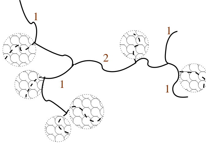
FIG. 3. “Snipped” priority (Read and McLeish, 2001) for the same molecule as in fig 2 at a certain flow rate. The segments having relaxation times shorter than the inverse flow rate are replaced by ‘blobs’ signifying localised frictional drags.
