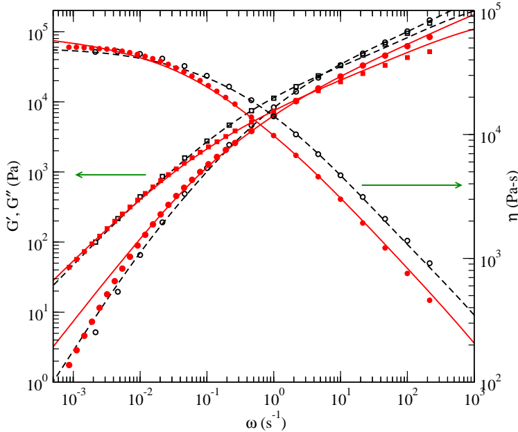
FIG. 7. Visco-elastic moduli and complex viscosity from small angle oscillatory shear experiments (symbols) and predictions (lines) for LDPE2 (filled symbols and solid lines) and HDB6 (open symbols and dashed lines).
