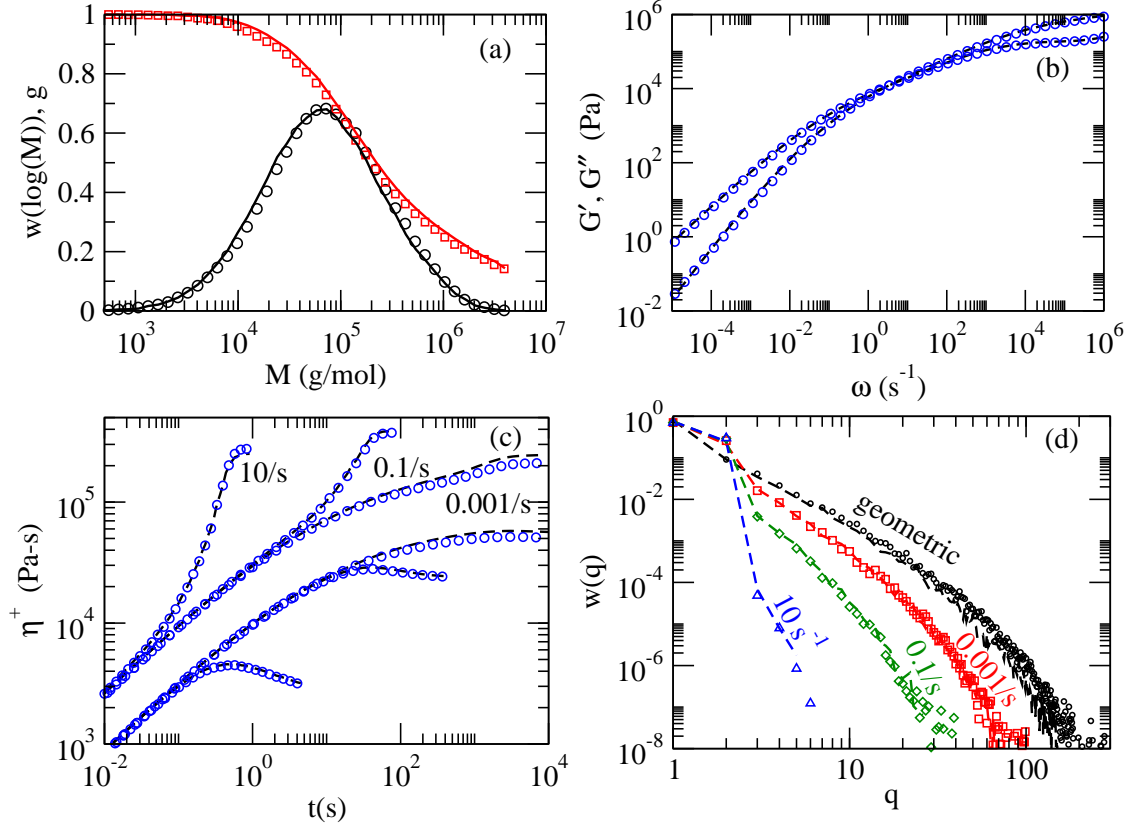
FIG. 9. Predictions for two different set of parameters for modelling LDPE2: (a) Distribution of molar mass and g-factor. Results from set1 are shown as symbols and from set2 are shown as lines. (b) Frequency dependence of the viscous and the elastic moduli for set1 (symbols) and set2 (dashed line) are virtually indistinguishable. (c) Start-up stress growth coefficients behave similarly for set1 (symbols) and set2 (dashed lines) in both extension (upper curves) and shear (lower curves) at the indicated flow rates. (d) Priority distributions for set1 (symbols) and set2 (dashed lines) behave similarly at the different flow rates.
