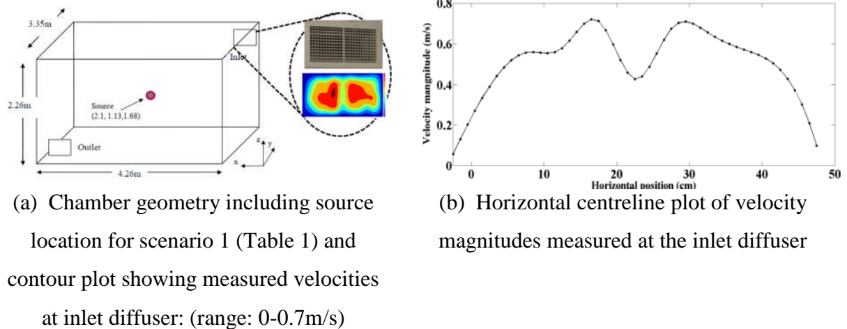
Fig. 1 Chamber geometry including centreline air speeds at the inlet
