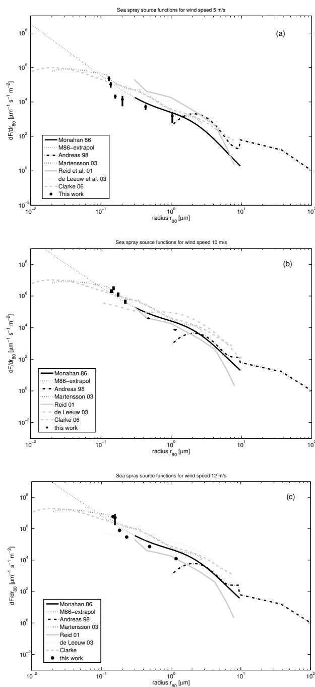
Fig. 6. Comparison of results from this work with a few sea spray source functions available in the literature for a number of different wind speeds (a) 5 \text{m s}^{-1} , (b) 10 \text{m s}^{-1} , (c) 12 \text{m s}^{-1} .
