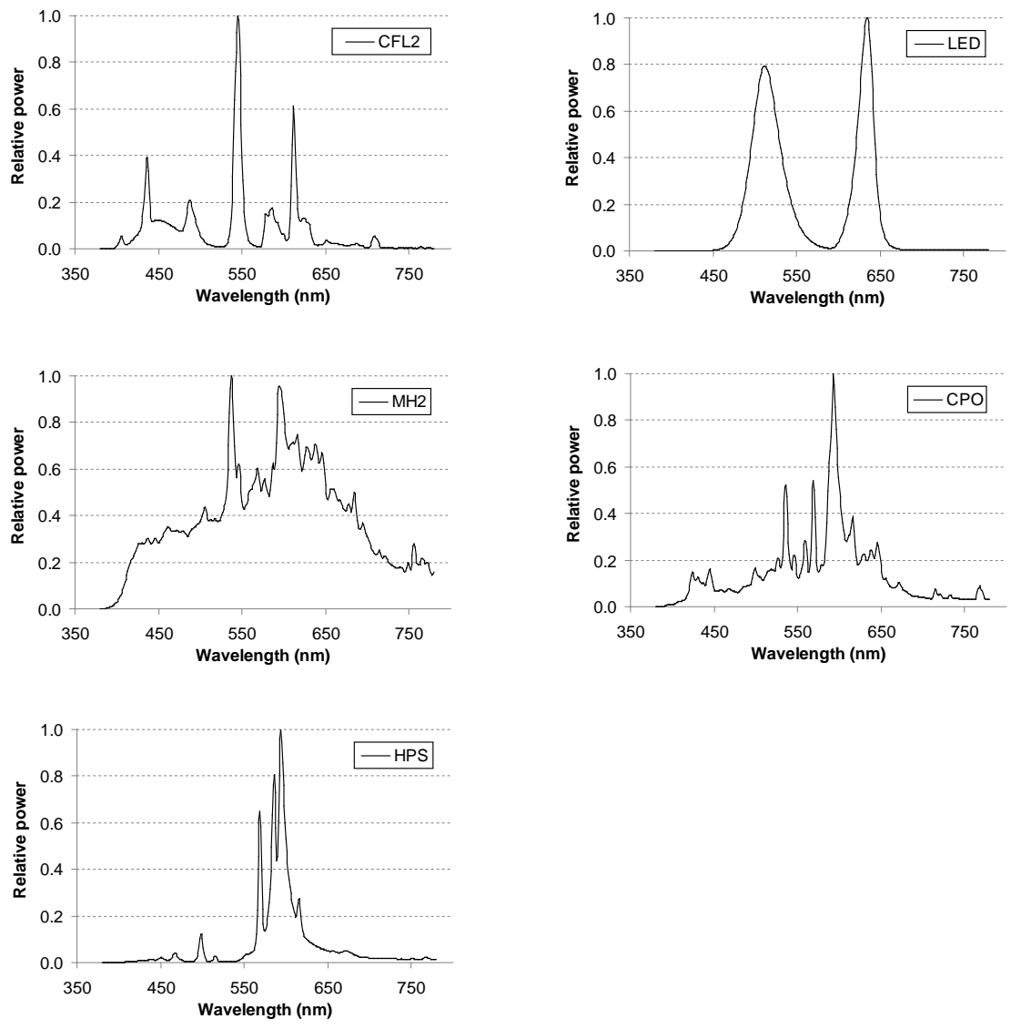
Figure 2 Spectral power distributions of the test lamps. These are as measured from the observers view point and hence include modification by the test apparatus, and are normalised for a peak response of 1.0.
