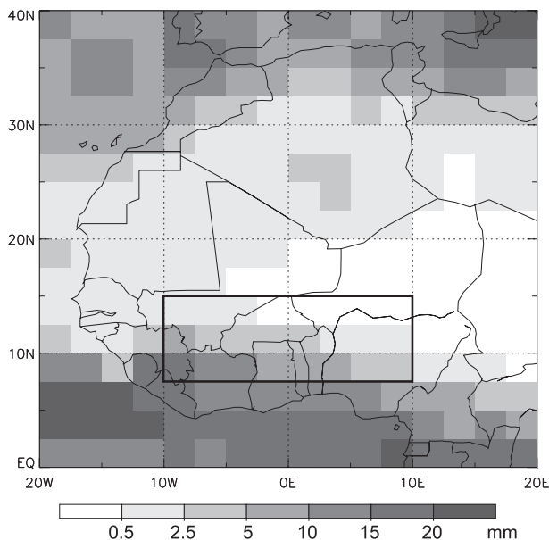
FIG. 6. Composed GPCP precipitation over all 43 wet events identified in section 4, in millimeters per pentad. A black box marks the study area.
