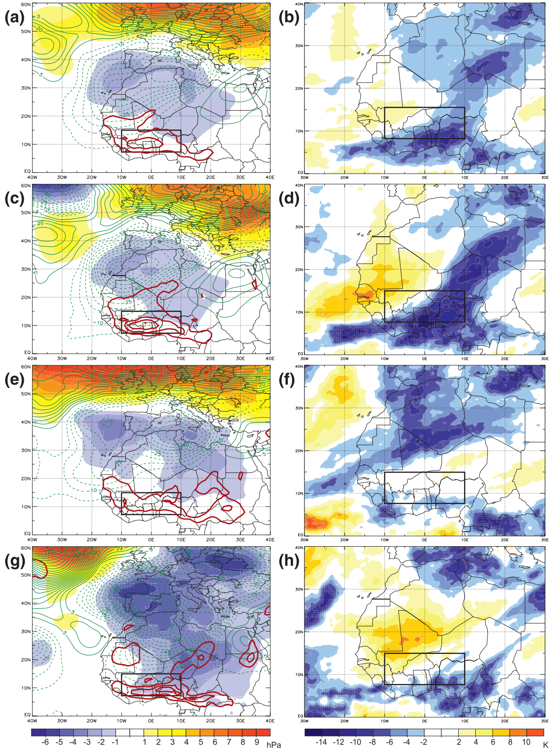
FIG. 12. Composites anomalies of (left) analyzed Z500 (contoured every 5 gpm), MSLP (shaded), and TD2M (red contours showing 2°, 4°, 6°, and 8°C) as well as (right) CLAUS BTs for day 0 over (a),(b) all 43 wet events, (c),(d) all 23 hits, (e),(f) all 20 misses, and (g),(h) all 11 false alarms. No CLAUS data are available before 1983, so these composites consist of (b) 35 events, (d) 20 events, and (f) 15 events. The false alarms are not affected. Black boxes mark the study area. Note the different geographical areas in the right and left panels.
