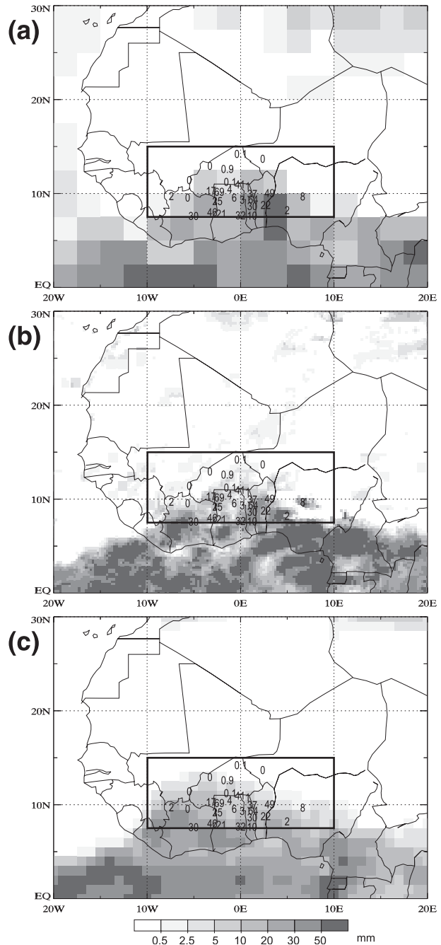
FIG. 1. 5-day accumulated precipitation during the pentad 15–19 Feb 1999 (in mm) from (a) GPCP, (b) TRMM, and (c) ERA-40 forecast data. Observations from selected rain gauges are indicated as numbers, with 0 indicating traces of rain. Black boxes mark the study area.
