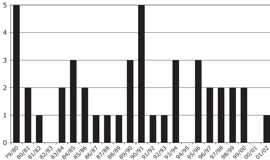
FIG. 5. Number of precipitation events for the 23 dry seasons from 1979/80 to 2001/02 as identified from GPCP pentad data using the routine described in section 4a.
