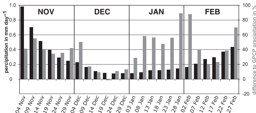
FIG. 7. Black bars show the mean annual cycle of precipitation as in Fig. 3 but based upon 5-day ERA-40 precipitation forecasts. The gray bars indicate the differences between the ERA-40 and GPCP data in %.
