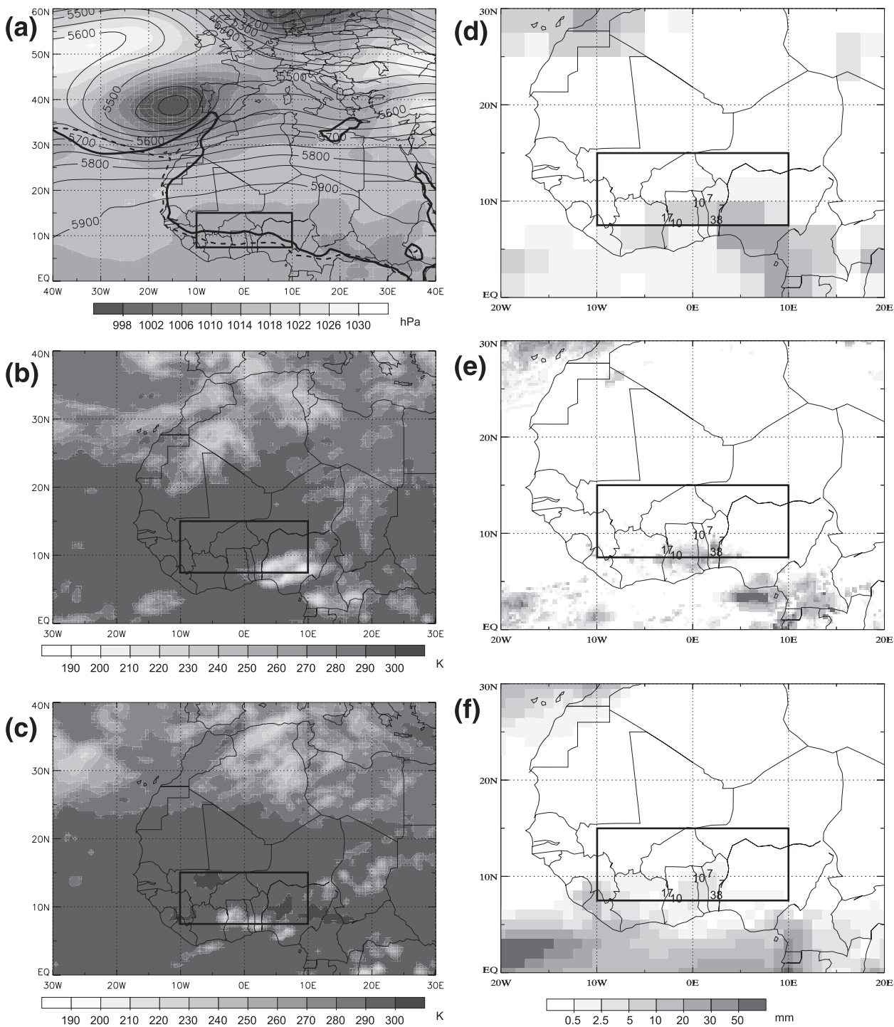
FIG. 13. Example of a forecast miss. (a) Analyzed Z500 (contours every 50 gpm), MSLP (shading), and 14°C contour of TD2M (thick solid line) at 1200 UTC 2 Feb 1998. The dashed line shows the 1979–2002 February average of the latter contour as a reference. (b),(c) CLAUS IR BTs at 2100 UTC on 1 and 2 February, respectively. (d)–(f) As in Fig. 1 but for 31 Jan–4 Feb 1998. Black boxes mark the study area.
