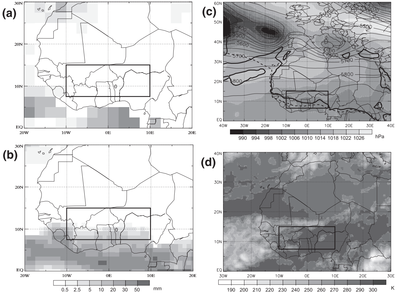
FIG. 10. Example of an extreme false alarm. The 5-day accumulated precipitation during the pentad 6–10 Jan 1997 (mm) from (a) ERA-40 forecast data and (b) GPCP. Only the synoptic station Djougou reported traces of precipitation during this period. (c) Analyzed Z500 (contours every 50 gpm), MSLP (shading), and 14°C contour of TD2M (thick solid line) at 1200 UTC 7 Jan 1997. The dashed line shows the 1979–2002 January average of the latter contour as a reference. (d) CLAUS IR BTs at 2100 UTC 7 Jan 1997. Black boxes mark the study area.
