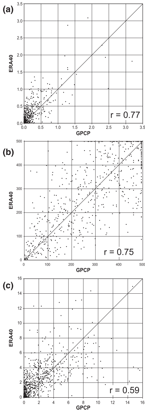
FIG. 8. Scatterplots relating pentad precipitation data from GPCP (abscissas) to ERA-40 5-day forecasts (ordinates) for the 552 pentads from 2 Nov to 1 March 1979/80–2001/02. (a) Area averages for 7.5^{\circ} – 15^{\circ} N, 10^{\circ} W– 10^{\circ} E ( \text{mm day}^{-1} ). (b) Ranking of the area averages shown in (a). Rank 494 in the GPCP data and rank 499 in the ERA-40 data correspond to zero precipitation. (c) As in (a) but for the 2.5^{\circ} \times 2.5^{\circ} gridbox maxima. The linear correlation coefficient r is given in each panel. All correlations are significant at the 99.9% significance level.
