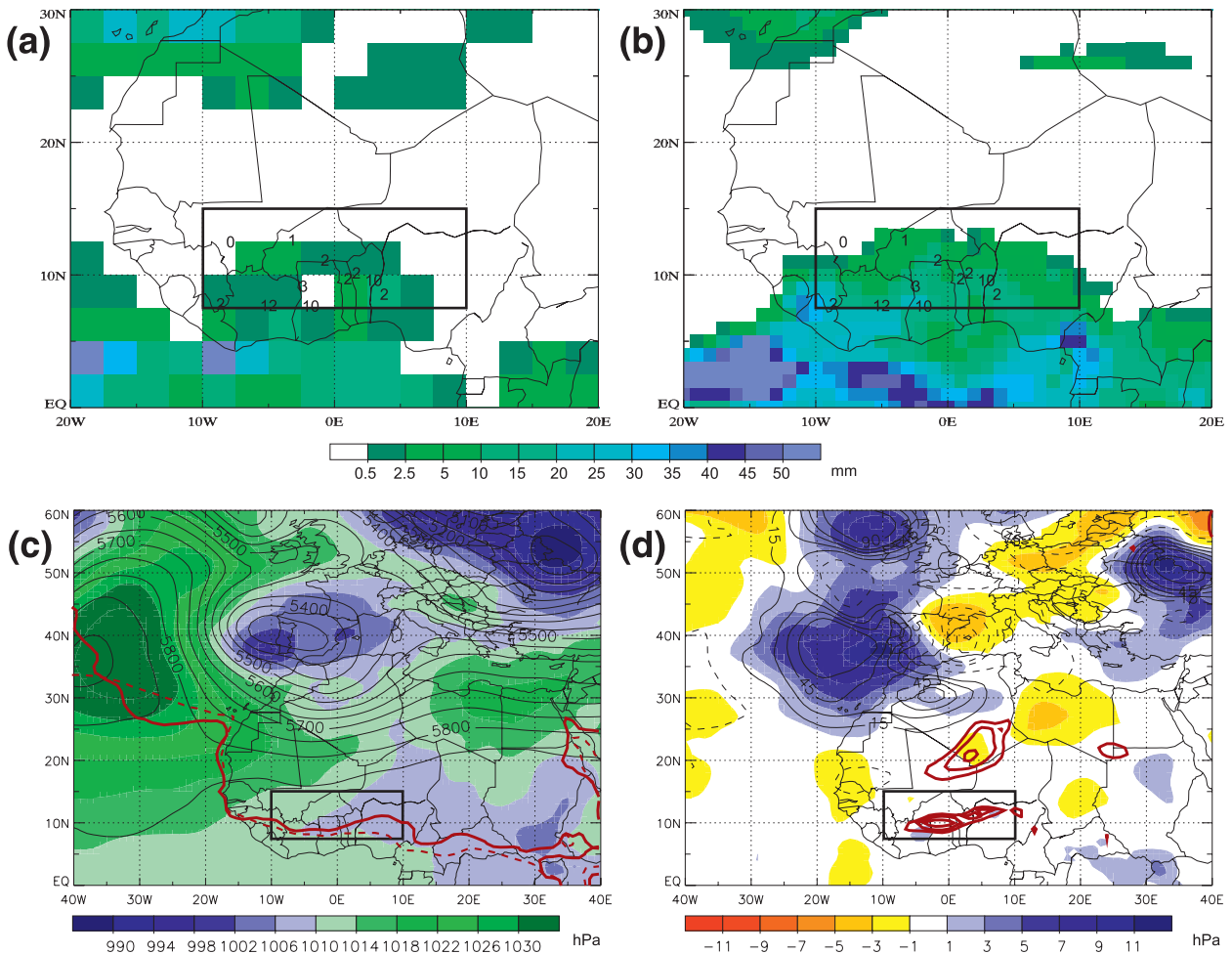
FIG. 15. Example of a false alarm. (a),(b) As in Figs. 1a and 1c but for 15–19 Feb 1991. (c) Z500 (contours every 50 gpm), MSLP (shading), and 14°C contour of TD2M (red solid line) at 1200 UTC 17 Feb 1991. The dashed red line shows the 1979–2002 February average of the latter contour as a reference. (d) Differences of Z500 (contoured every 15 gpm), MSLP (shaded), and TD2M (red contours showing 6°, 10°, and 14°C) between the 60-h forecast from ERA-40 valid at 1200 UTC 17 Feb 1991 and the corresponding reanalysis. Black boxes mark the study area.
