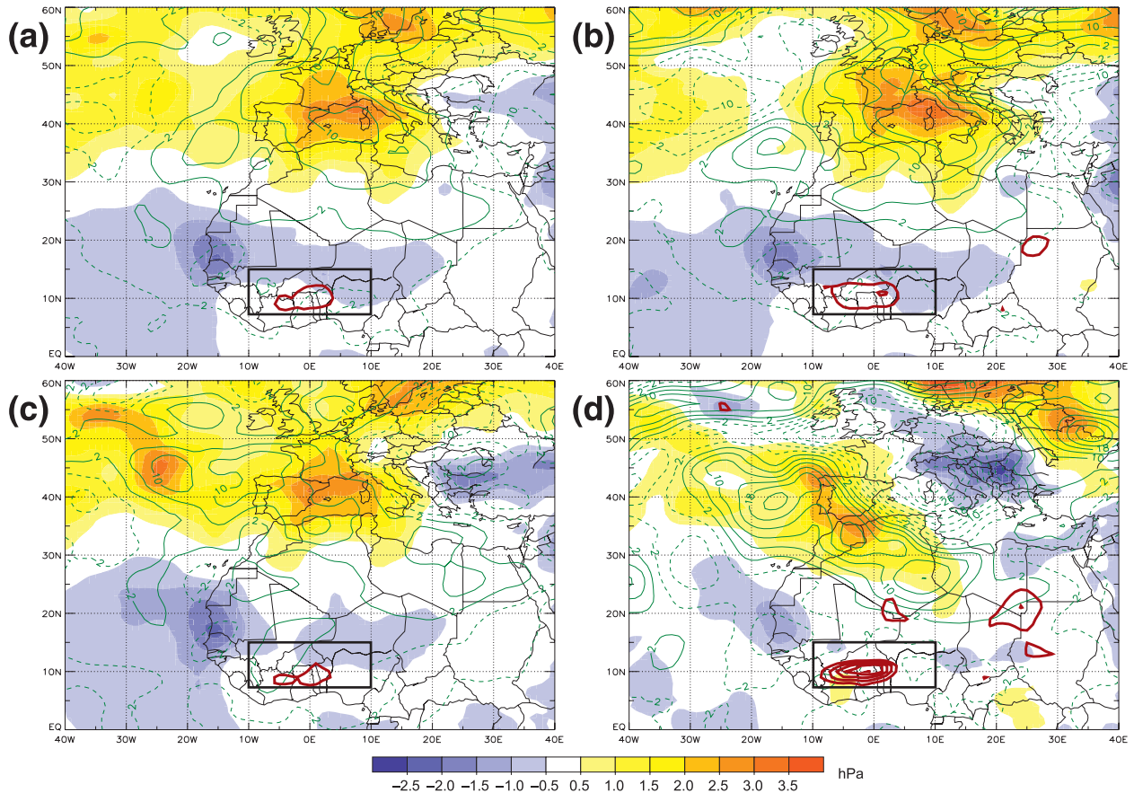
FIG. 14. Composites differences of Z500 (green contours every 4 gpm), MSLP (shaded), and TD2M (red contours showing 2°, 4°, 6°, 8°, and 10°C) between the 60-h forecasts from ERA-40 and the corresponding reanalysis for day 0: (a) all 43 wet events, (b) all 23 hits, (c) all 20 misses, and (d) all 11 false alarms. Black boxes mark the study area.
