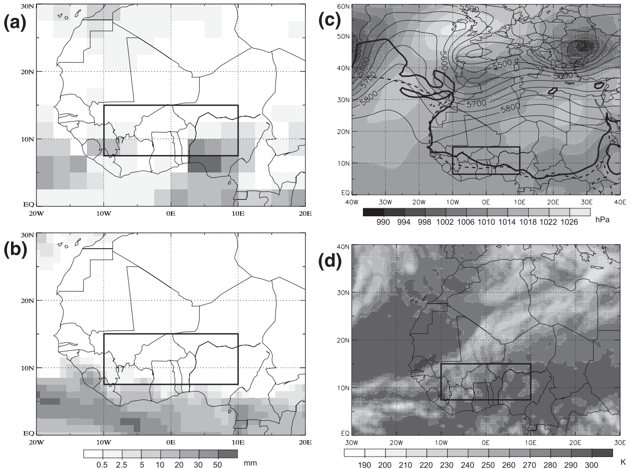
FIG. 9. Example of an extreme forecast miss. The 5-day accumulated precipitation during the pentad 2–6 Dec 1997 (mm) from (a) ERA-40 forecast data and (b) GPCP. Only the synoptic station Odienne reported precipitation during this period. (c) Analyzed Z500 (contours every 50 gpm), MSLP (shading), and 14°C contour of TD2M (thick solid line) at 1200 UTC 4 Dec 1997. The dashed line shows the 1979–2001 December average of the latter contour as a reference. (d) CLAUS IR BTs at 2100 UTC 4 Dec 1997. Black boxes mark the study area.
