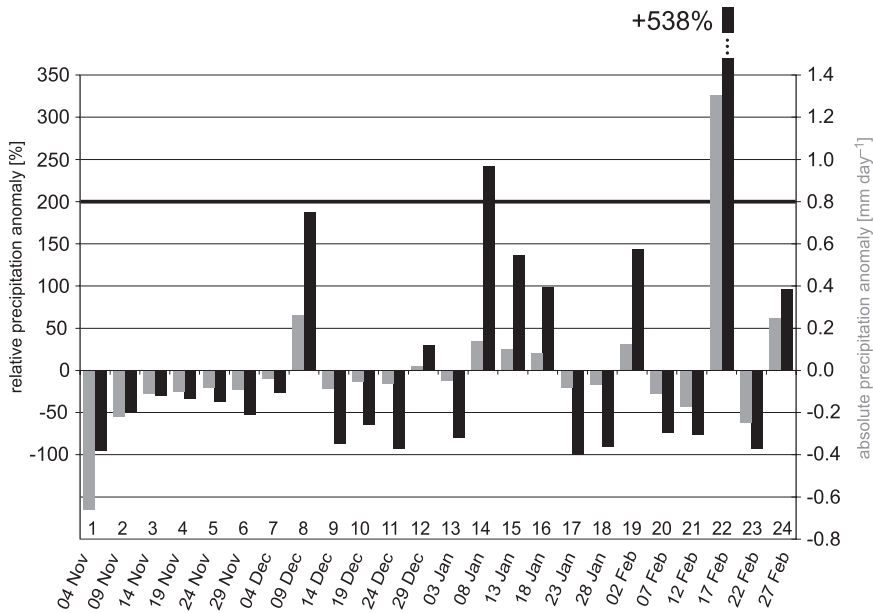
FIG. 4. Pentad precipitation anomalies over the area 7.5°–15°N, 10°W–10°E during the West African dry season of 2 Nov 1998–1 Mar 1999. Anomalies were calculated with respect to the mean pentad values displayed in Fig. 3 and expressed in mm day -1 (gray bars, right ordinate) and in % (black bars, left ordinate), respectively. The dates along the abscissa give the center day of the respective pentad, which are numbered serially for reference in the text.
