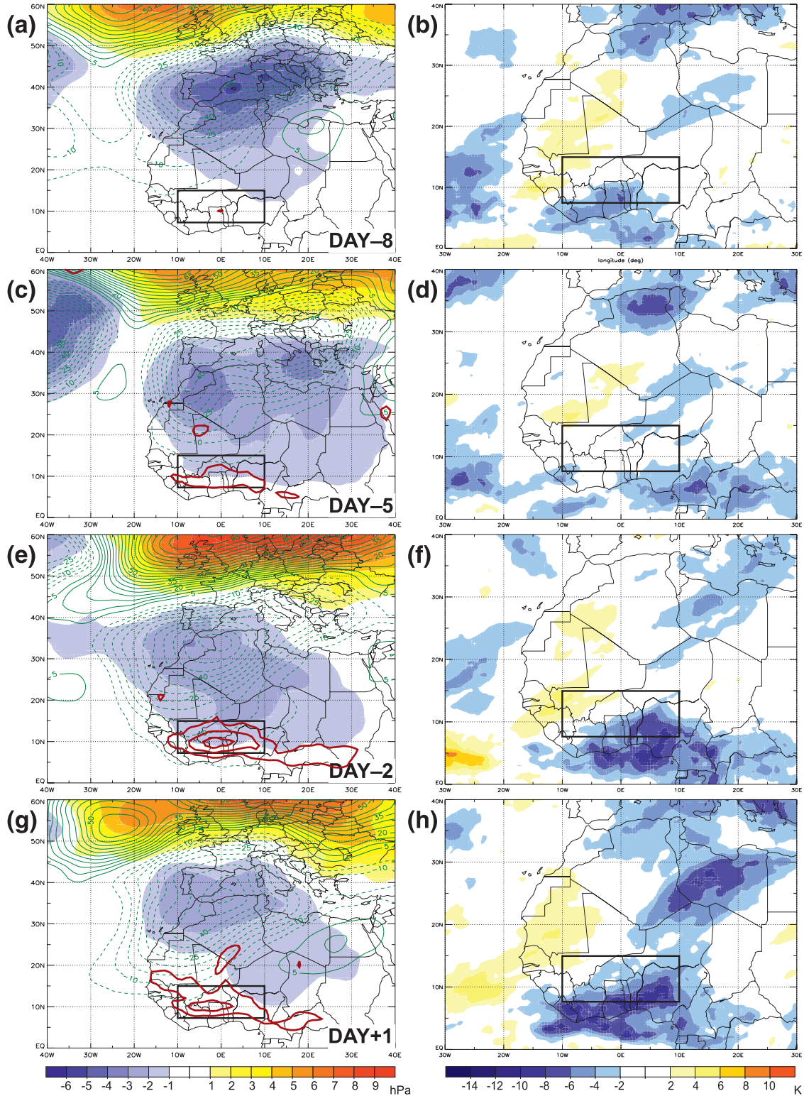
FIG. 11. Composites anomalies of (left) Z500 (green contours every 5 gpm), MSLP (shaded), and TD2M (red contours showing 2°, 4°, and 6°C) as well as (right) CLAUS IR BTs over all 43 wet events identified in section 4b for (a),(b) day -8, (c),(d) day -5, (e),(f) day -2, and (g),(h) day +1. No CLAUS data are available before 1983, so these composites consist of only 35 events. Black boxes mark the study area. Note the different geographical areas in the right and left panels.
