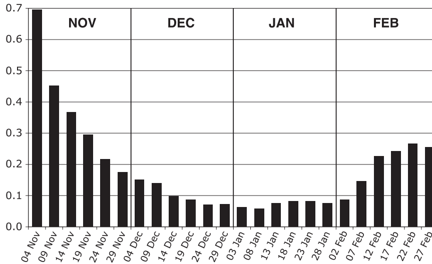
FIG. 3. Mean pentad precipitation ( \text{mm day}^{-1} ) over the area 7.5^{\circ}\text{--}15^{\circ}\text{N} , 10^{\circ}\text{W--}10^{\circ}\text{E} during the West African dry season of 2 November–1 March based upon GPCP pentad precipitation estimates of the 23 dry seasons from 1979/80 to 2001/02. The dates along the abscissa give the center day of the respective pentad. Months are defined as in Table 1.
