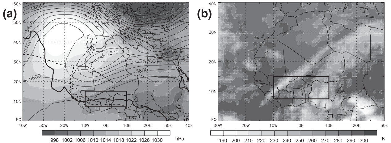
FIG. 2. (a) Z500 (contours every 50 gpm), MSLP (shading), and 14^{\circ}\text{C} contour of TD2M (thick solid line) at 1200 UTC 17 Feb 1999. The dashed line shows the 1979–2002 February average of the latter contour as a reference. (b) The CLAUS IR brightness temperatures at 2100 UTC on this day. Black boxes mark the study area.
