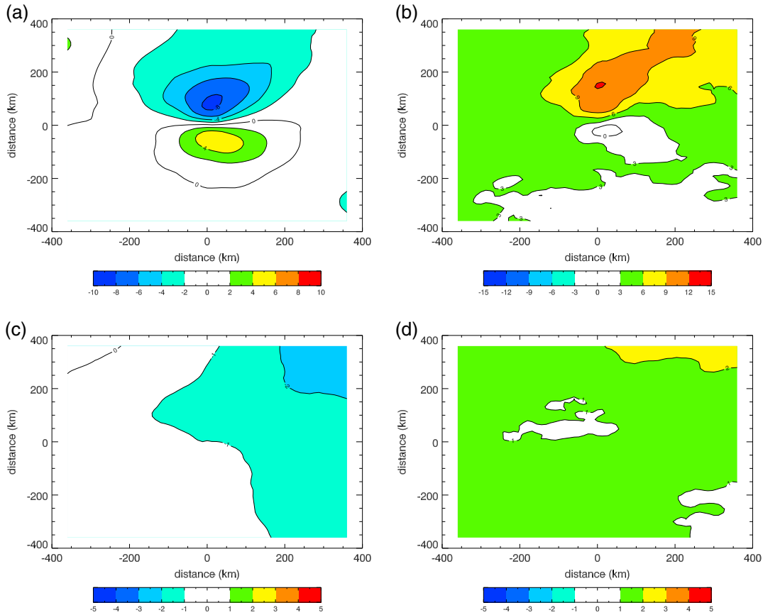
Figure 3. Composites around surface rainfall of (a, c) eddy heat fluxes ( v'\theta' ) and (b, d) cooling by meridional advection ( v \cdot d\theta/dy ). Figures 3a and 3b are for 12kmExp and Figures 3c and 3d for 12kmParam (all at 320 m above the ground). Note different color scales.
