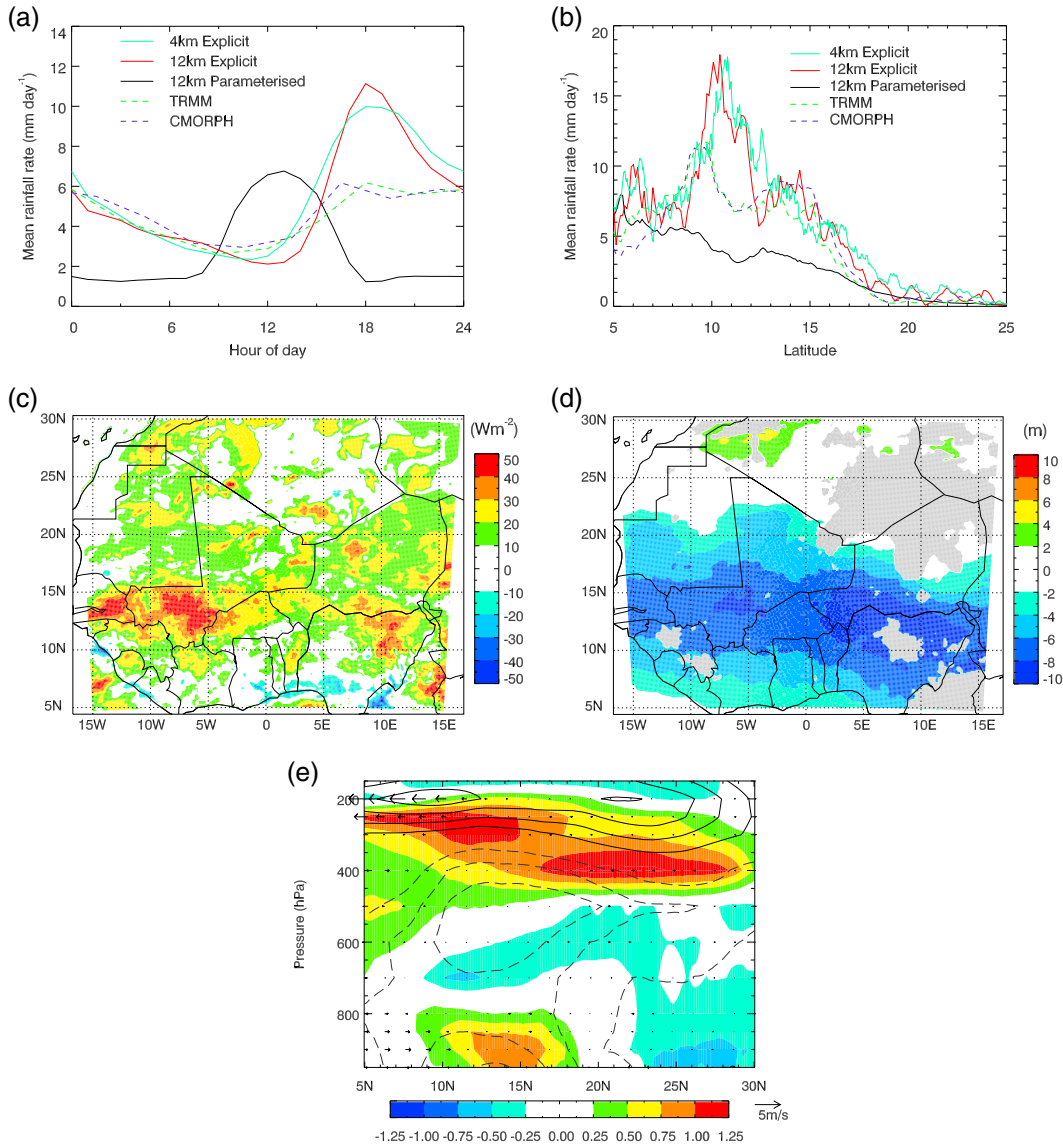
Figure 1. (a) Diurnal cycle in rain in 12kmParam, 12kmExp, and 4kmExp and from TRMM and CMORPH retrievals, averaged over 5°N to 25°N and 10°W to 10°E. (b) Mean latitudinal distributions of rain for the same runs and the same longitudes. The 12kmExp-12kmParam difference in (c) net surface radiation, (d) 950 hPa geopotential height (grey shows orography intersecting the 950 hPa surface), and (e) vertical cross section of geopotential height (lines with 2 m spacing; the dashed lines are negative) and potential temperature (colors; K) over 10°E to 10°W.
