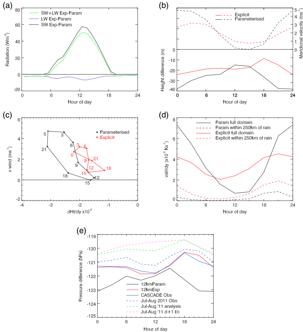
Figure 2. Differences in the diurnal cycle between 12kmParam and 12kmExp: (a) surface radiation ( 12^{\circ}\text{N} to 24^{\circ}\text{N} and 10^{\circ}\text{W} to 10^{\circ}\text{E} ); (b) 950 hPa geopotential height difference between the Sahel and the Sahara ( 12^{\circ}\text{N} to 24^{\circ}\text{N} ) and meridional winds (dashed) over 10^{\circ}\text{W} to 10^{\circ}\text{E} ; (c) 950 hPa geopotential gradient between the Sahel and the Sahara and meridional winds. (d) Total cooling by meridional advection ( v \cdot d\theta/dy ) over 13^{\circ}\text{N} to 25^{\circ}\text{N} and 10^{\circ}\text{W} to 8^{\circ}\text{E} (solid lines) and over this domain and within 250 km of rain (dashed lines); (e) pressure difference between Tamanrasset ( 22.8^{\circ}\text{N} 5.5^{\circ}\text{E} ) and Niamey ( 13.5^{\circ}\text{N} 2.1^{\circ}\text{E} ): observed ( Cascade period in 2006 and in July and August 2011), in Cascade runs (2006), and in UM analyses and forecasts (July and August 2011; 6 hourly with T+6 to T+24 ). Offsets have been applied to account for the height differences between the surface stations and equivalent model grid boxes.
