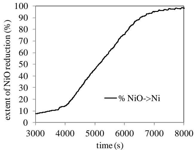
Fig 7 NiO reduction vs. time (% of NiO fresh catalyst), S:C=4, T=750 °C, cycle 2
