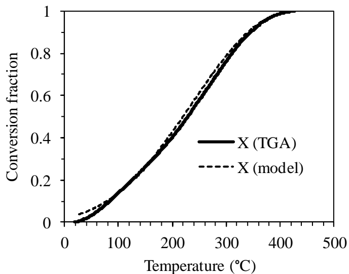
Fig 2 Conversion fraction of STPO vs. temperature during TGA (50 ml/min N 2 , 3 K min -1 ). Kinetic model curve corresponds to contracting volume (best fit), with A=5.93 \times 10^{-3} and E = 12.31 \pm 0.03 \text{ kJ mol}^{-1} , which produced a linear correlation of 0.9983.
