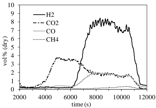
Fig. 5 \text{H}_2 , \text{CO}_2 , \text{CO} and \text{CH}_4 vol % in the dry reformat vs. time on stream from the steam reforming of STPO at S:C=4 and 750°C. Balance to 100 vol. % attributed to \text{N}_2 gas carrier, cycle 2.
