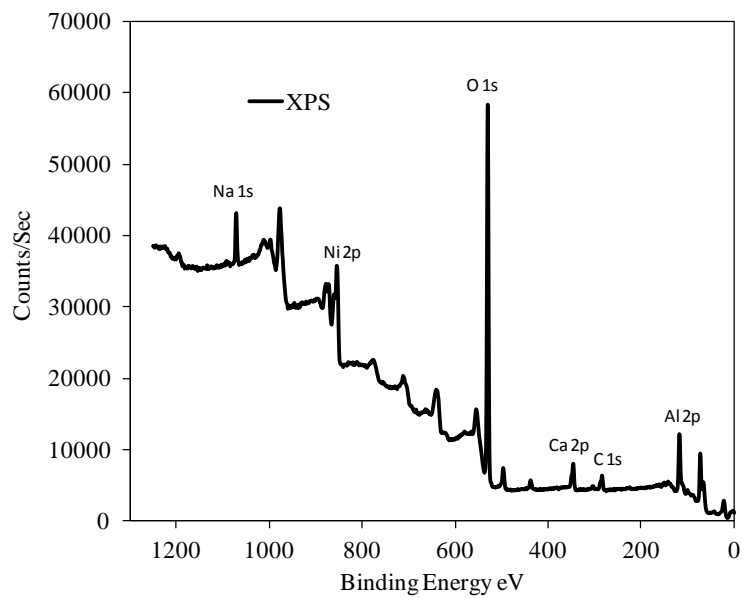
Fig. 9 XPS analysis of used NiO catalyst (cycle 4).
