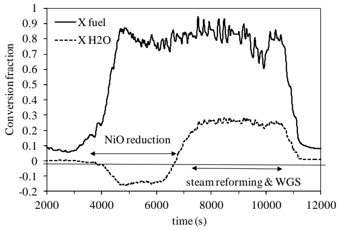
Fig. 6 Conversion of oil and water vs. time on stream during fuel-steam feed step, S:C=4,
