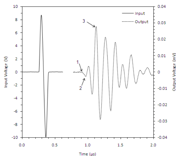
Figure 2. Typical oscilloscope signals from a bender element test with sine pulse excitation.
