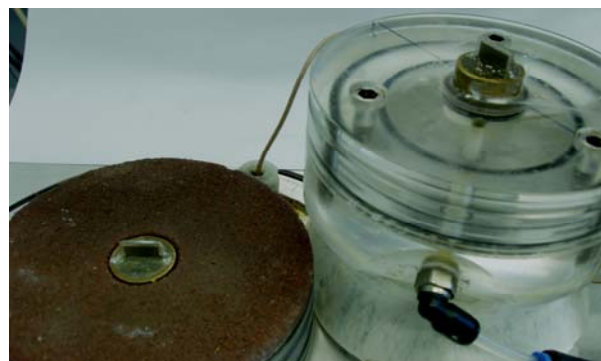
Figure 3. Bender element probes mounted into the triaxial test apparatus.
