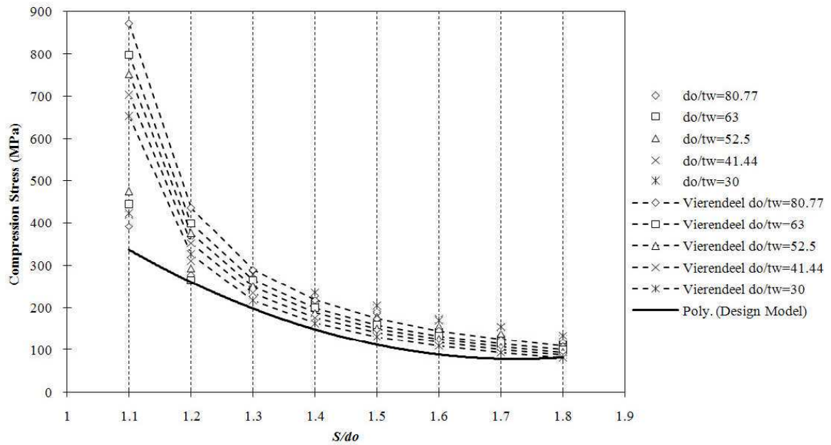
Fig. 12: Empirical design curve evaluating the compressive strength of the ‘strut’ (A1 & B1)
