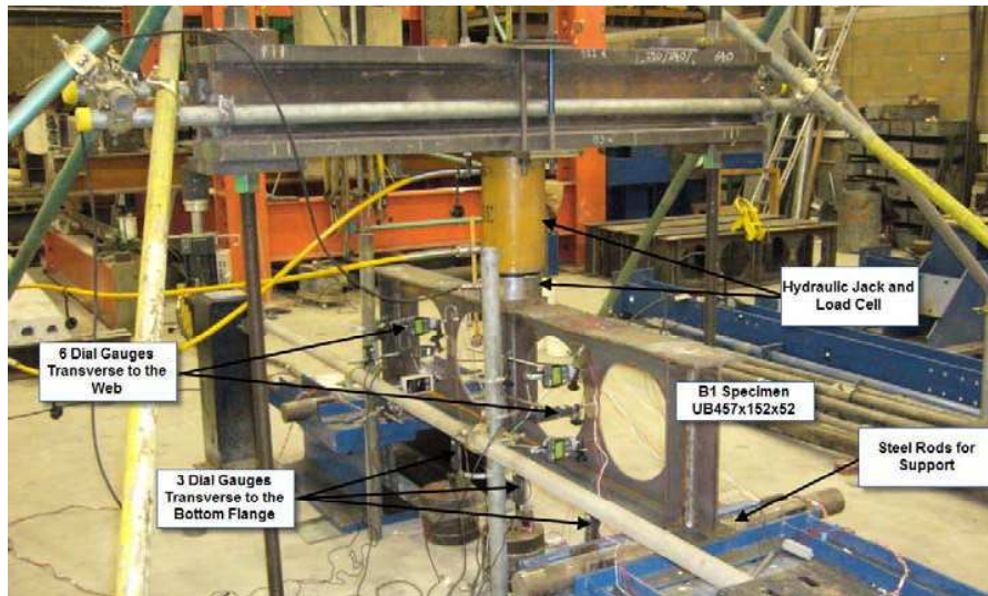
Fig. 2: Test set-up arrangement
