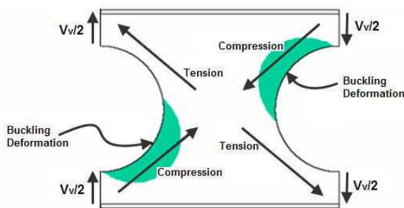
Fig. 7: Typical web-post behaviour
