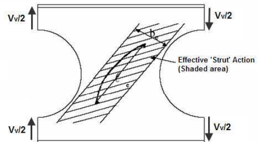
Fig. 8: Strut model of web-post buckling
