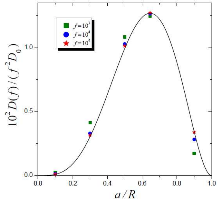
Figure 6. The effective diffusivity D(f) scaled by f^2 D_0 as a function of a/R . The solid line is calculated from eq 19. Points, marked by symbols described in the legend, are obtained from simulations at l/R = 2 .
