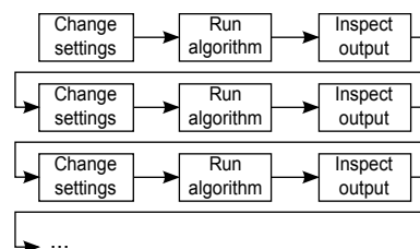
Fig. 1. The conventional approach for parameter optimization. Based on a qualitative assessment of current output, users iteratively change parameter settings and run algorithms to generate new output. This process is repeated until the output quality is satisfactory.
