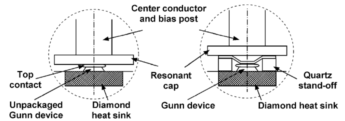
Fig. 4. Schematic of the WR-5/6 waveguide cavity for second-harmonic power extraction at G -band (140–220 GHz).
