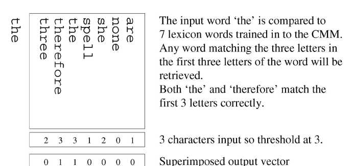
Fig. 6. Diagram showing Hamming Distance matching.
