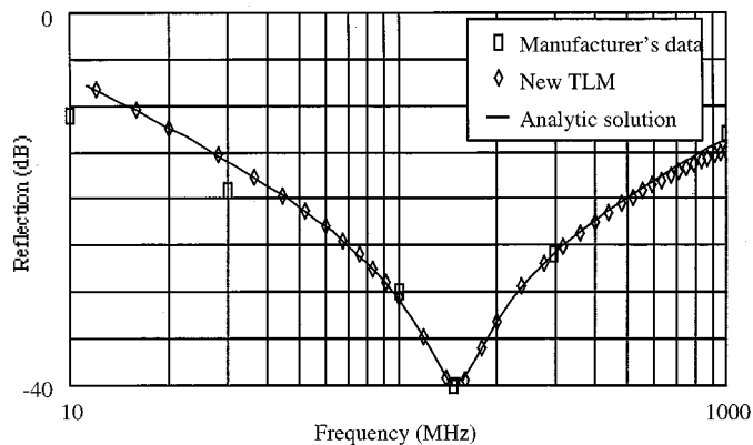
Fig. 4. Modeled reflectivity curve for Philips' tiles compared with analytic and manufacturer's data.
