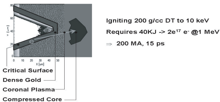
Figure 2. Ignition conditions and fast electron path in an FI target.
