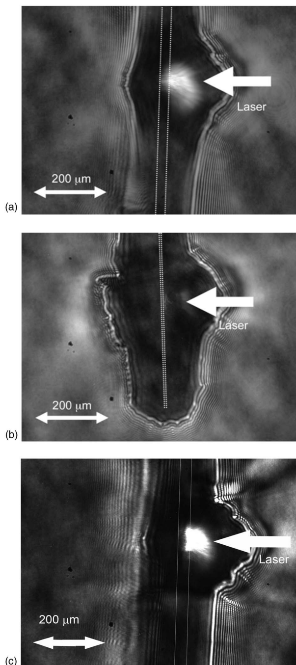
FIG. 2. (a) Shadowgraph of 25 \mu\text{m SiO}_2 + 1 \mu\text{m Cu} back layer taken at t_0 + 200 \text{ ps} . (b) Shadowgraph of 4 \mu\text{m Al} / 1 \mu\text{m Ni} / 1 \mu\text{m CH} taken at t_0 + 200 \text{ ps} . The dotted lines mark the position of the original target surfaces. (c) An example of 25 \mu\text{m CH} + 1 \mu\text{m Cu} back layer taken at t_0 + 200 \text{ ps} .
