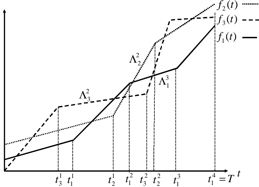
Figure 3: Example with three functions
