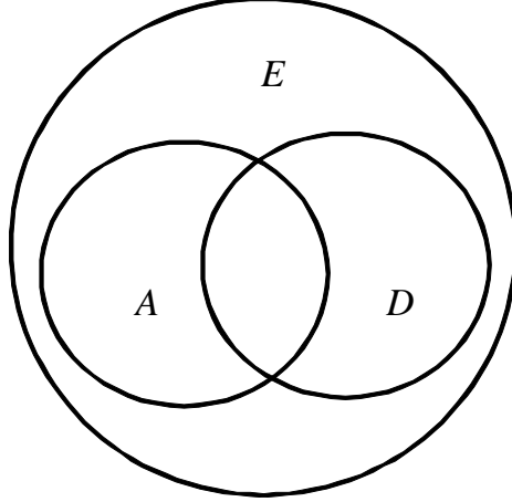
Figure 2: The structure of sets A, D and E
