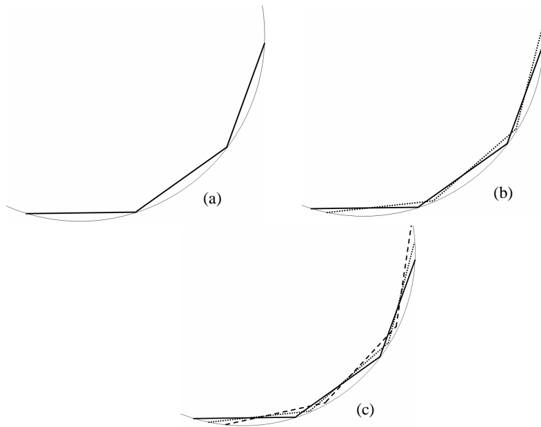
Figure 4: Generation of the tightness example: (a) one function, (b) two functions, (c) three functions
